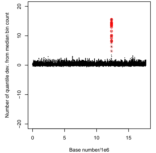
# Quant. Dev. from Median Bin Count; Chr. X
