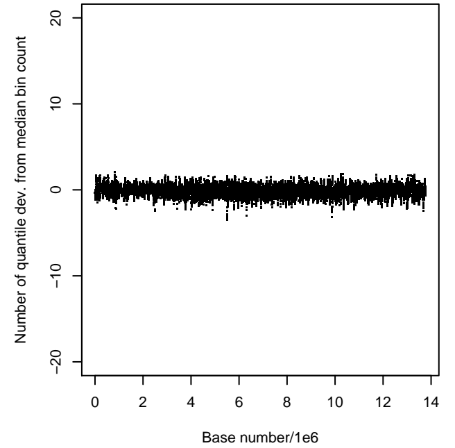
# Quant. Dev. from Median Bin Count; Chr. III
