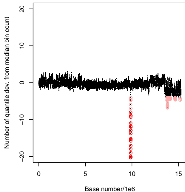
# Quant. Dev. from Median Bin Count; Chr. II
