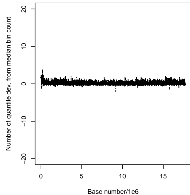
# Quant. Dev. from Median Bin Count; Chr. X
