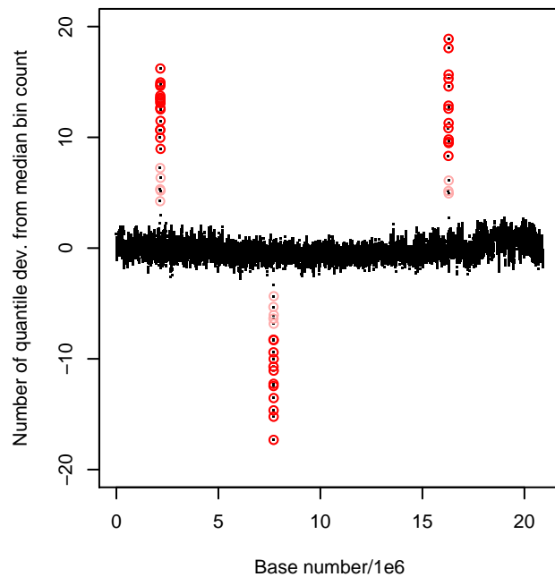
# Quant. Dev. from Median Bin Count; Chr. V
