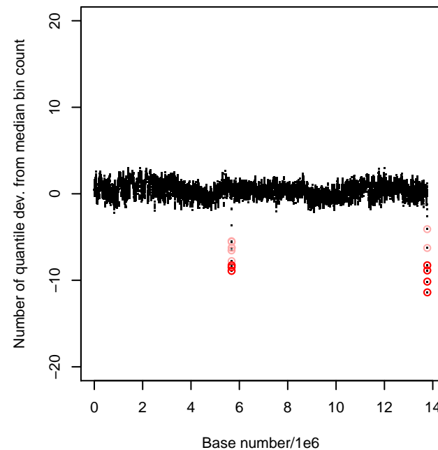
# Quant. Dev. from Median Bin Count; Chr. III
