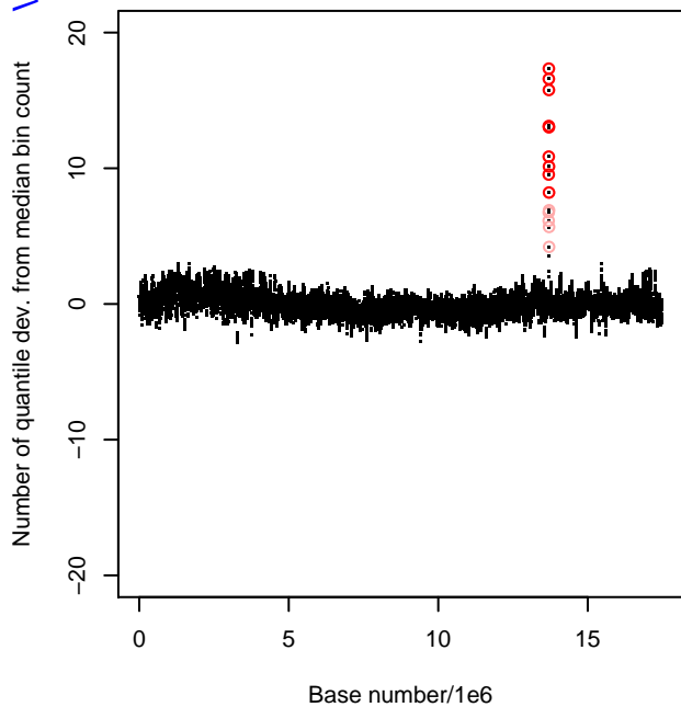
# Quant. Dev. from Median Bin Count; Chr. IV
