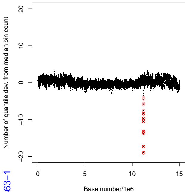
# Quant. Dev. from Median Bin Count; Chr. I
