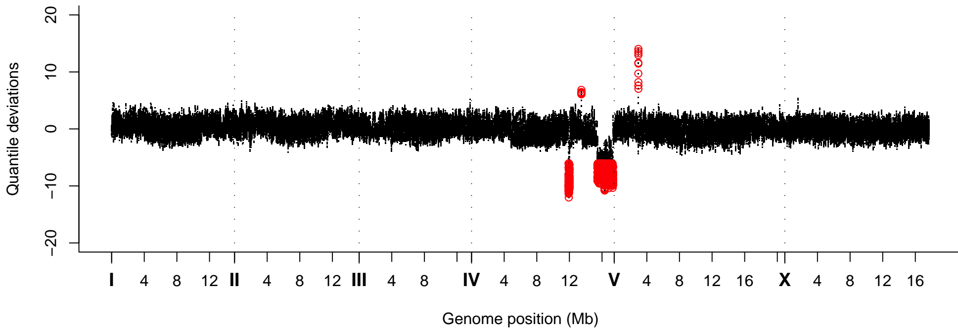
Quantile Deviations, Strain VC10129
