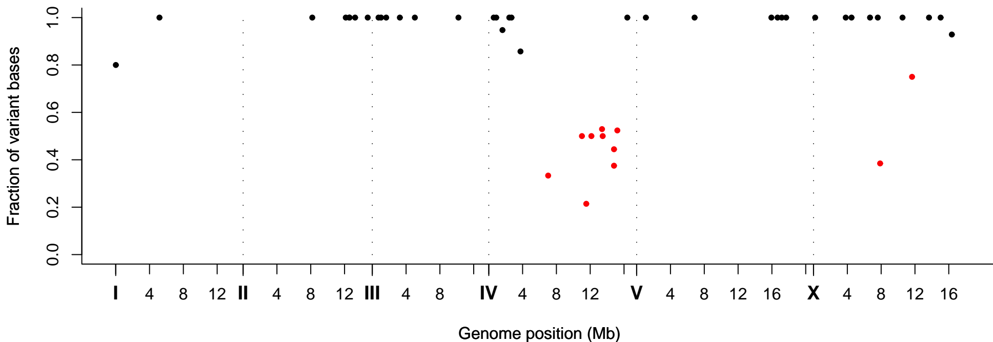
Fraction of Variant Bases at Position, Strain VC10129
