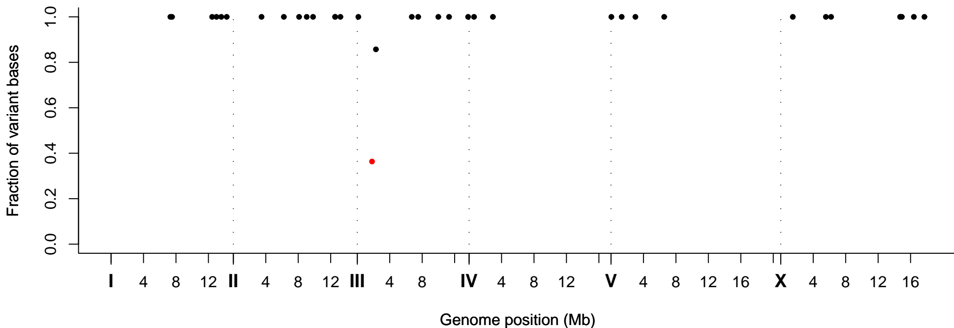
Fraction of Variant Bases at Position, Strain VC10165
