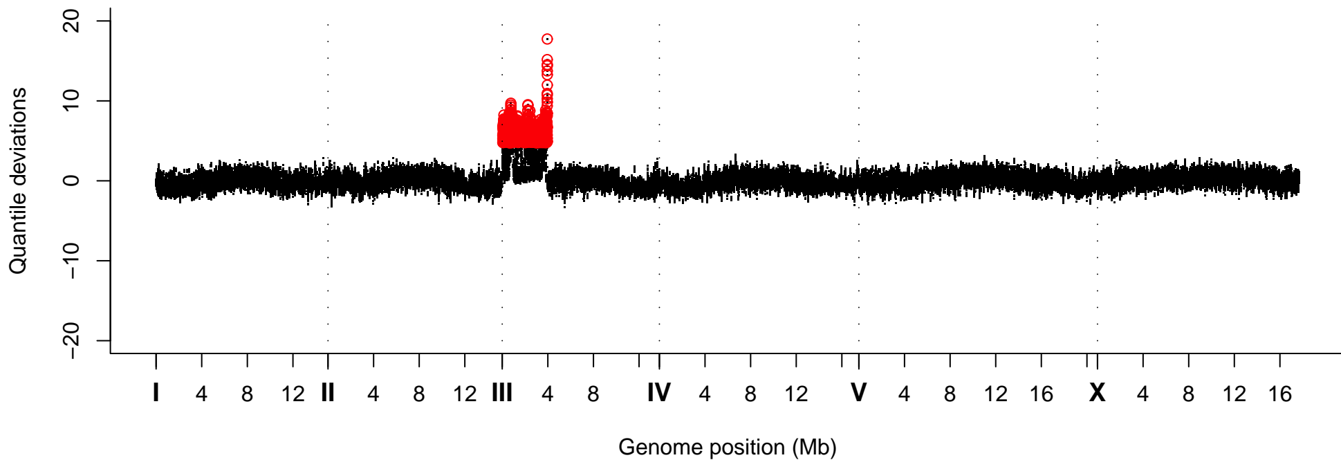
Quantile Deviations, Strain VC10165
