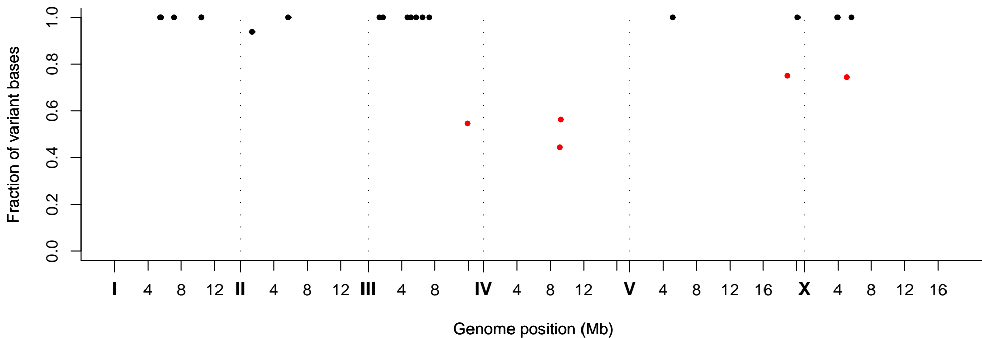
Fraction of Variant Bases at Position, Strain VC10166
