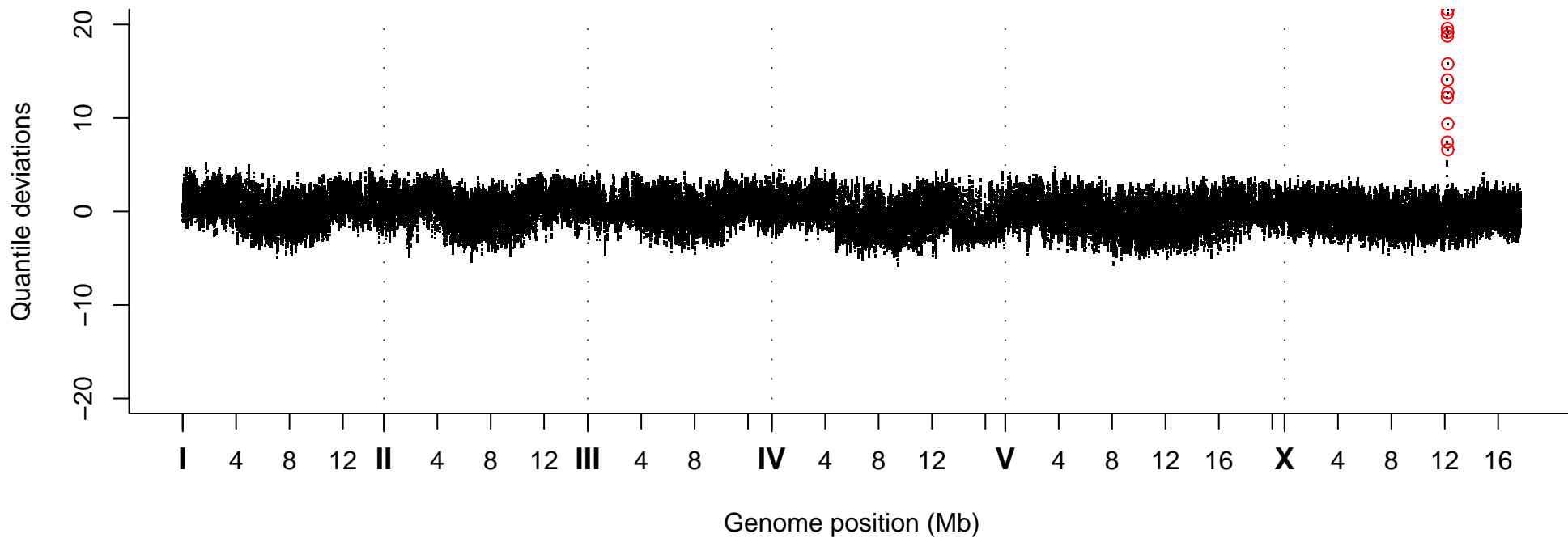
Quantile Deviations, Strain VC10166
