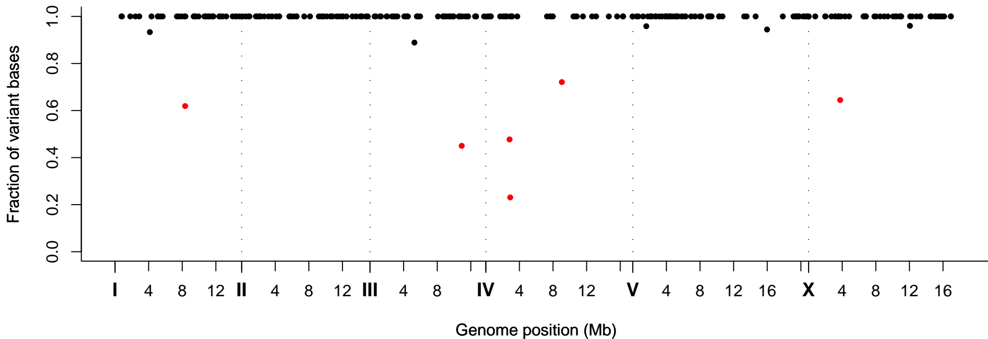
Fraction of Variant Bases at Position, Strain VC20011
