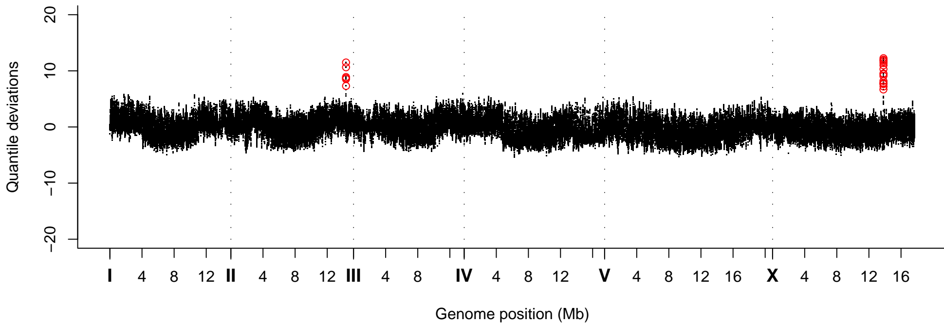
Quantile Deviations, Strain VC20011
