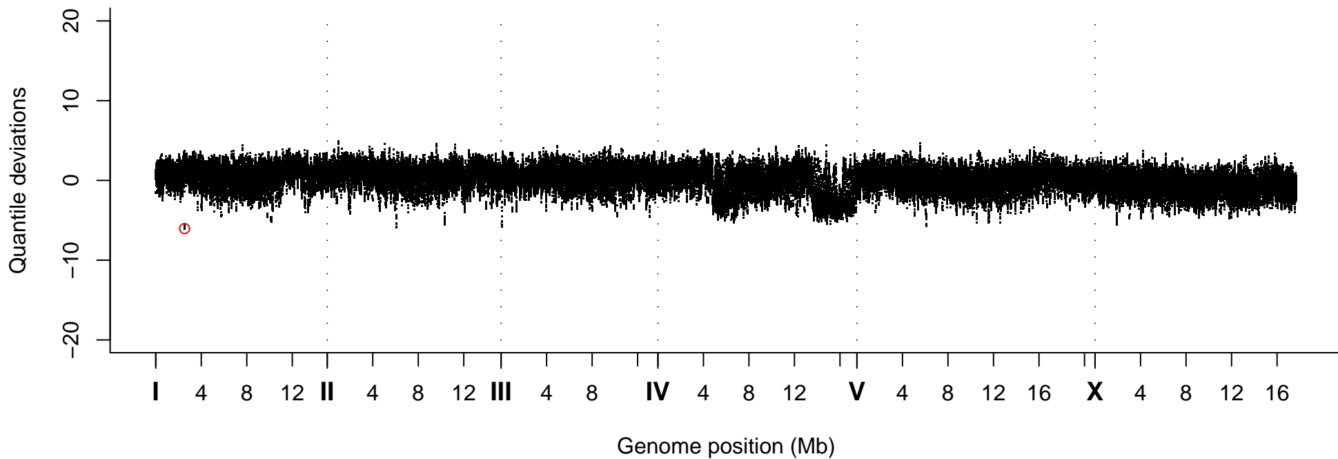
Quantile Deviations, Strain VC20026
