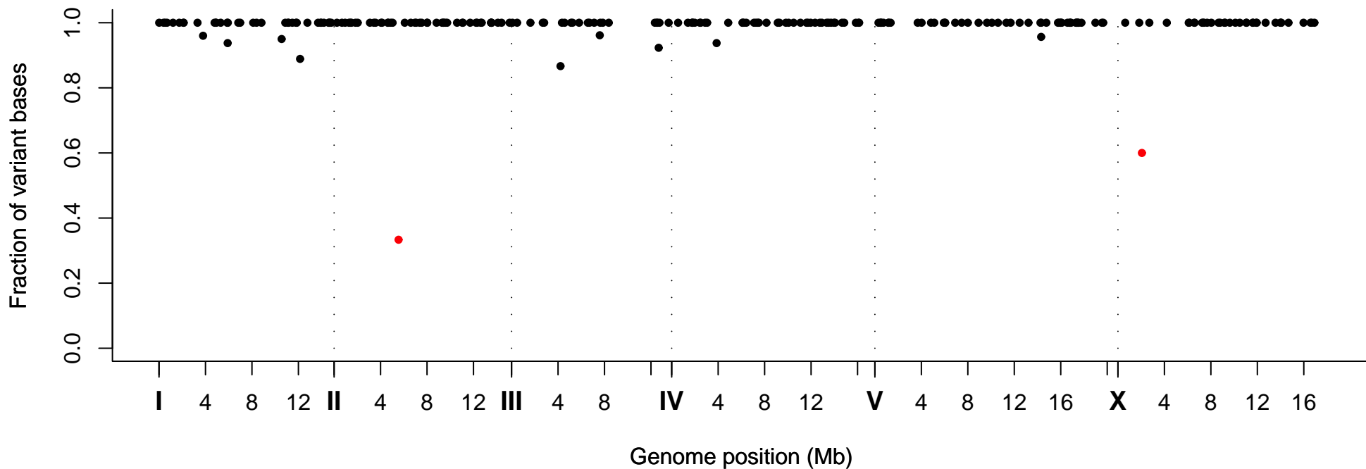
Fraction of Variant Bases at Position, Strain VC20026
