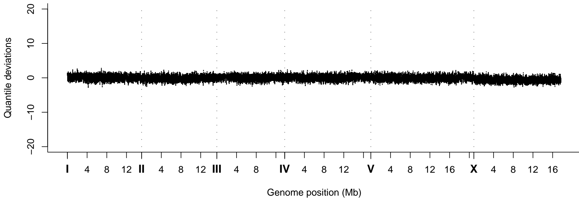
Quantile Deviations, Strain VC20030
