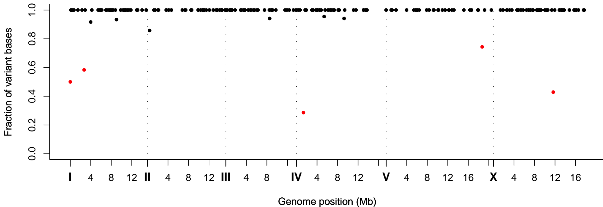
Fraction of Variant Bases at Position, Strain VC20030
