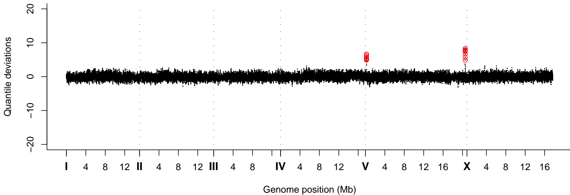
Quantile Deviations, Strain VC20043
