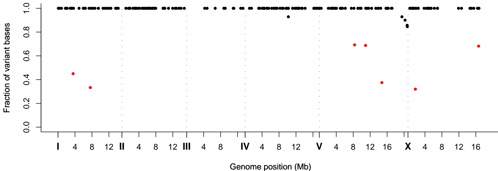
Fraction of Variant Bases at Position, Strain VC20043
