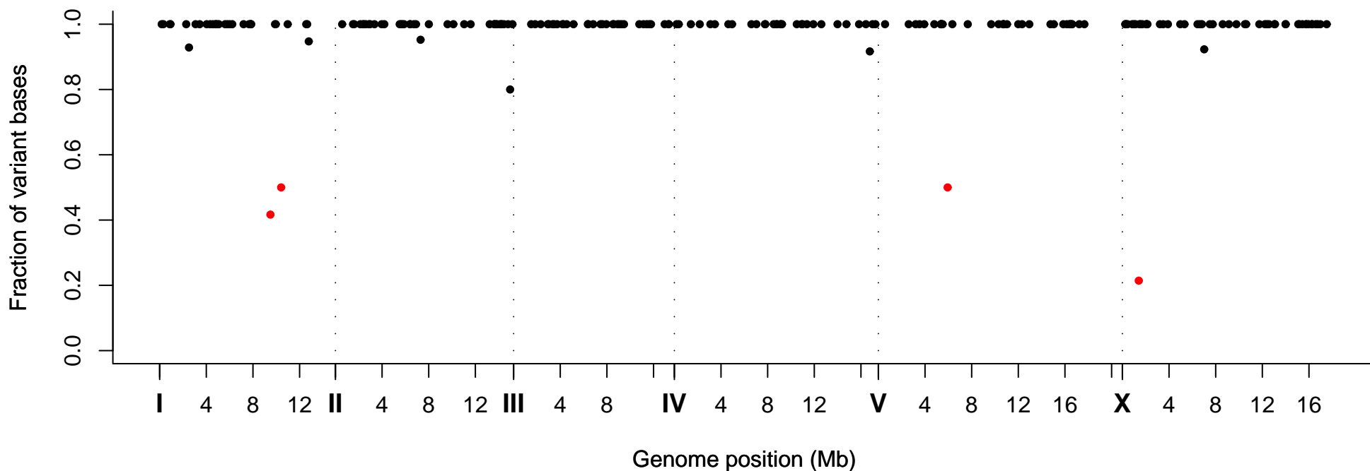
Fraction of Variant Bases at Position, Strain VC20044
