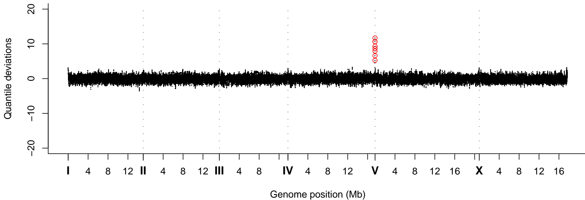
Quantile Deviations, Strain VC20044
