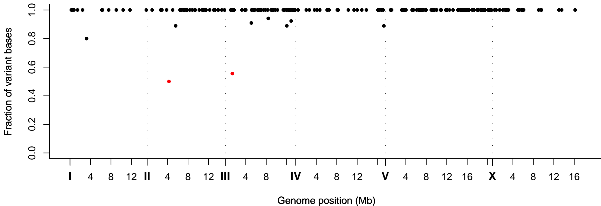
Fraction of Variant Bases at Position, Strain VC20045
