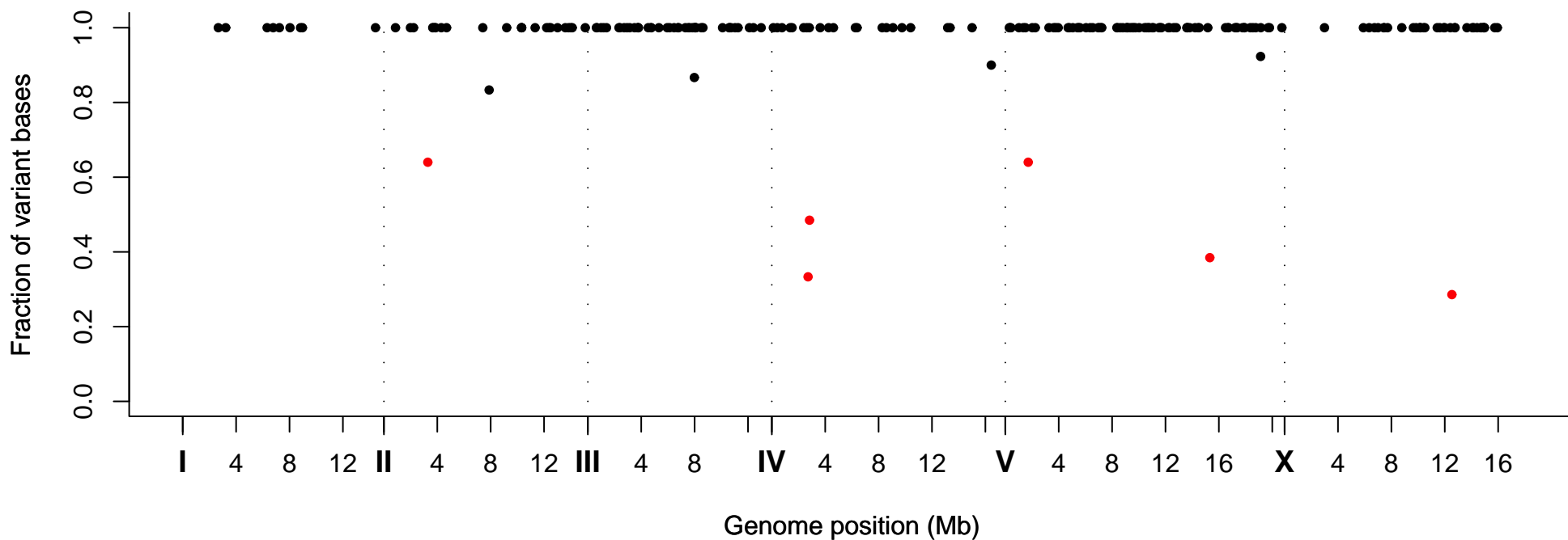
Fraction of Variant Bases at Position, Strain VC20048
