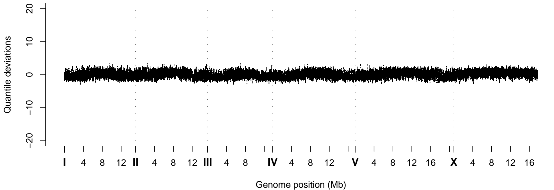
Quantile Deviations, Strain VC20048
