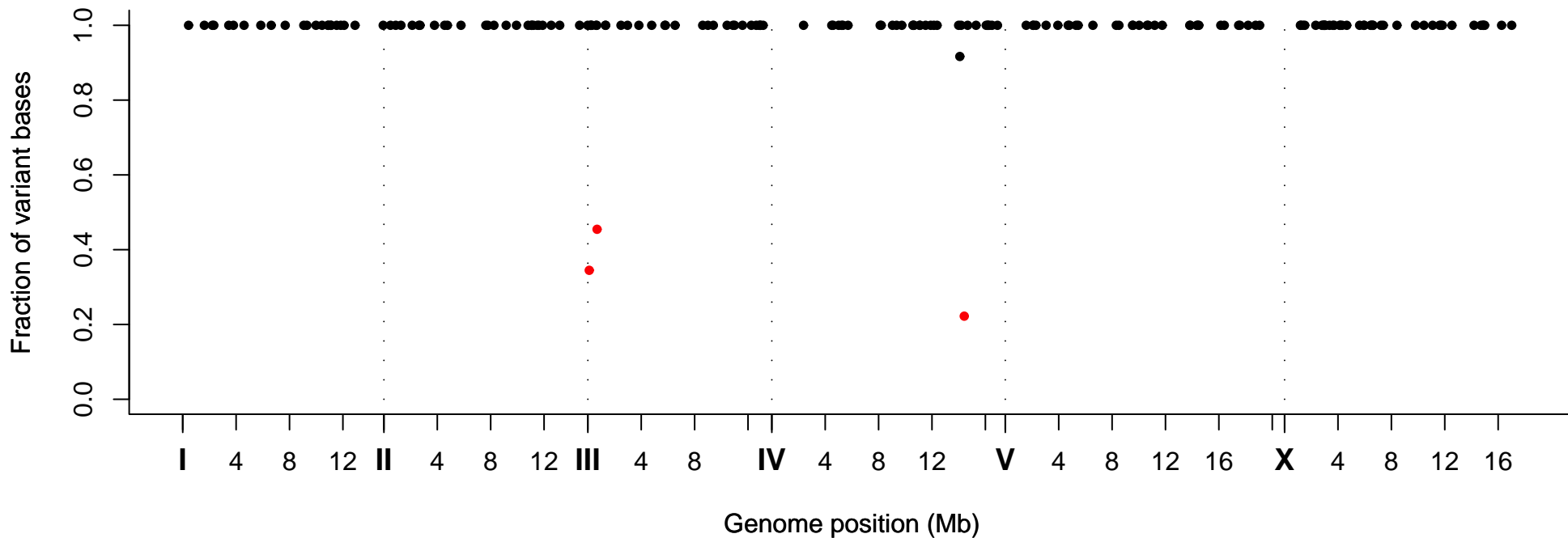
Fraction of Variant Bases at Position, Strain VC20051
