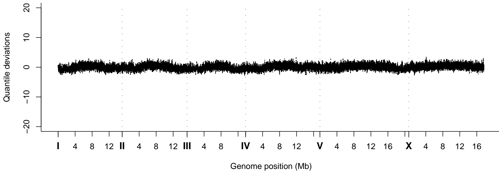
Quantile Deviations, Strain VC20051
