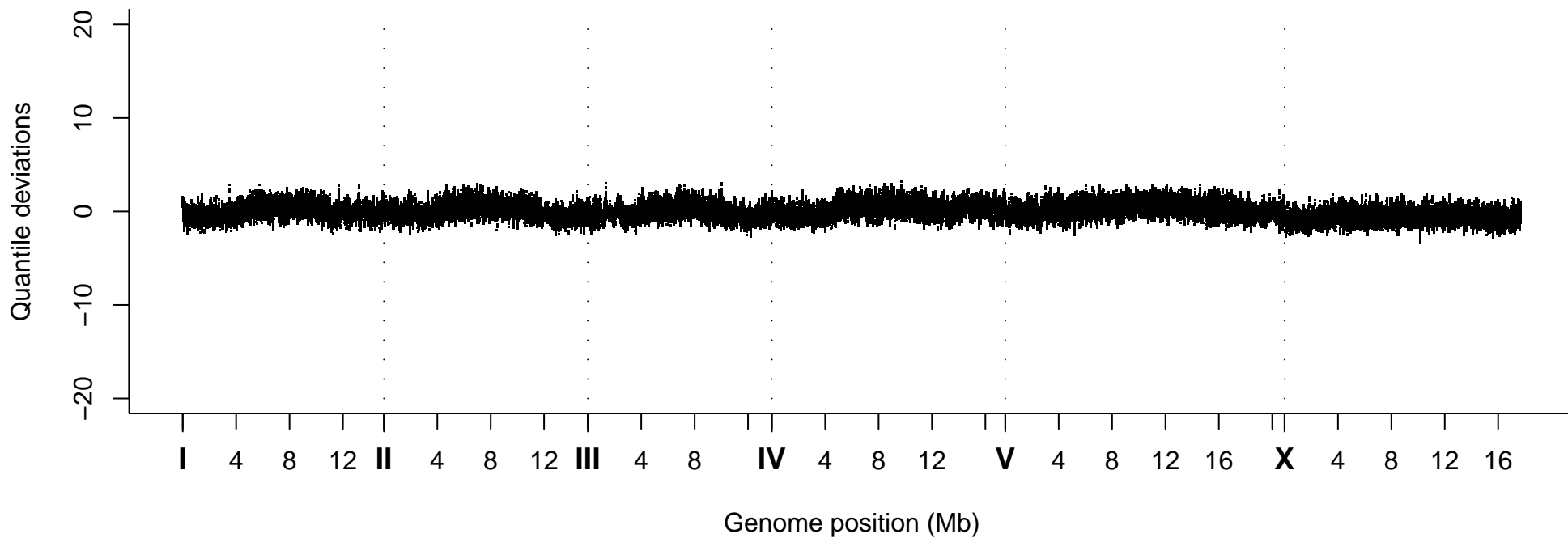
Quantile Deviations, Strain VC20052
