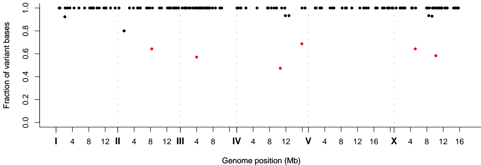
Fraction of Variant Bases at Position, Strain VC20052
