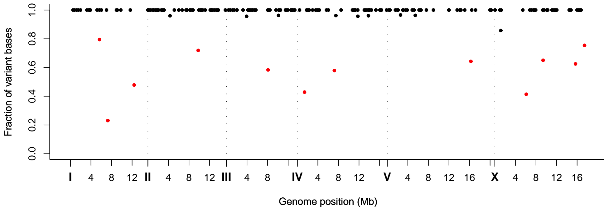
Fraction of Variant Bases at Position, Strain VC20054
