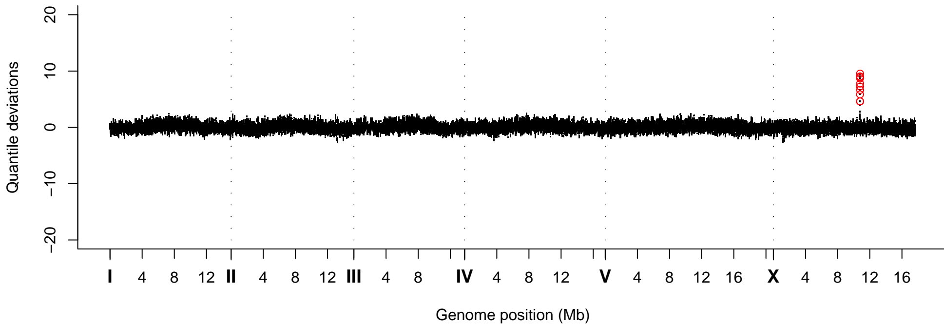
Quantile Deviations, Strain VC20054
