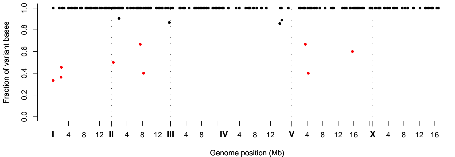
Fraction of Variant Bases at Position, Strain VC20055
