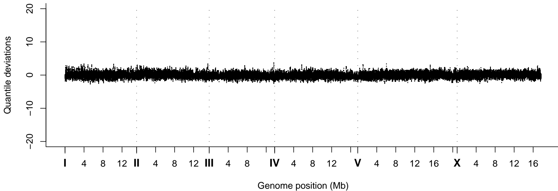
Quantile Deviations, Strain VC20055
