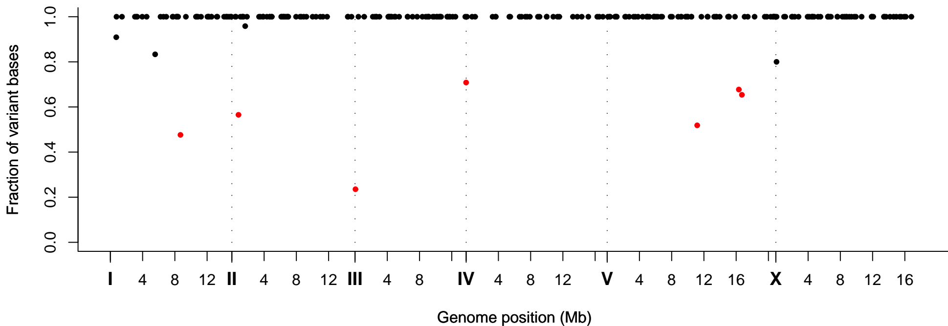
Fraction of Variant Bases at Position, Strain VC20057
