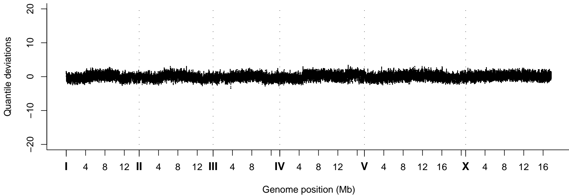
Quantile Deviations, Strain VC20057
