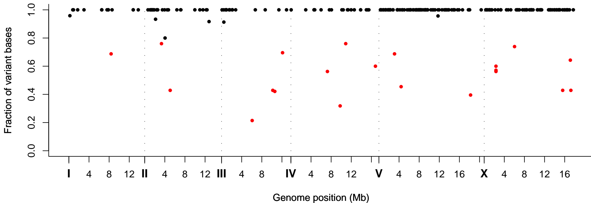
Fraction of Variant Bases at Position, Strain VC20058
