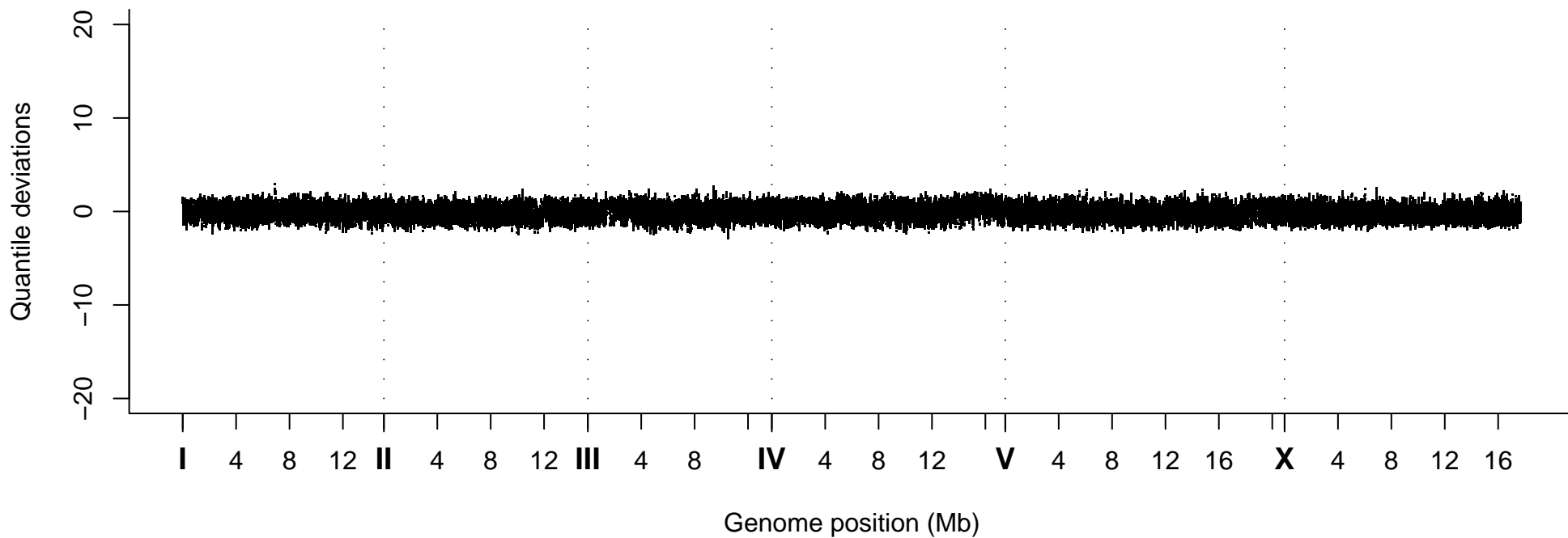
Quantile Deviations, Strain VC20058
