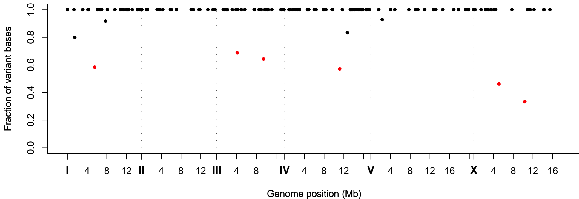
Fraction of Variant Bases at Position, Strain VC20061
