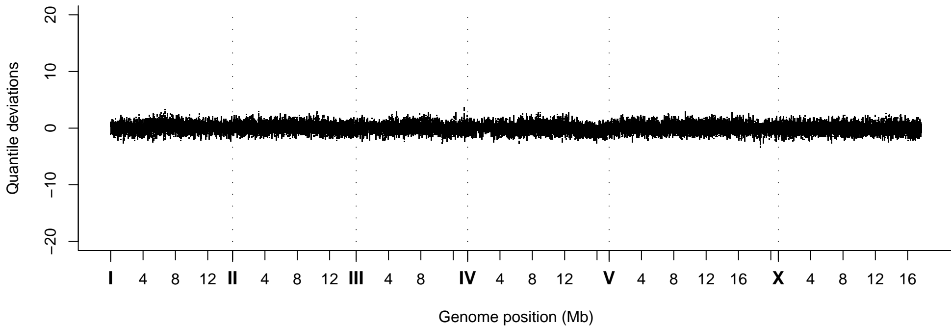
Quantile Deviations, Strain VC20061
