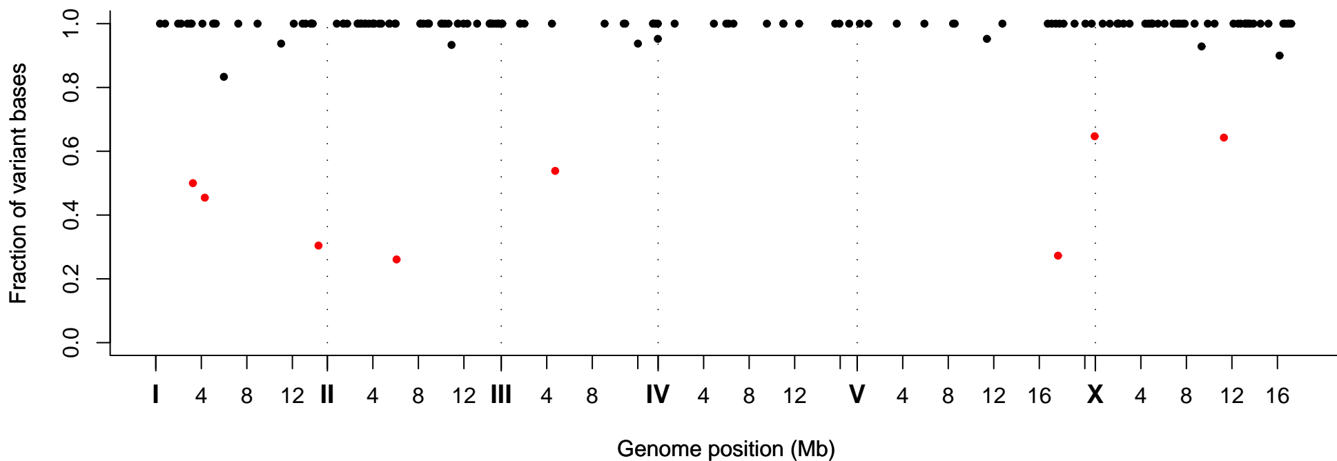
Fraction of Variant Bases at Position, Strain VC20062
