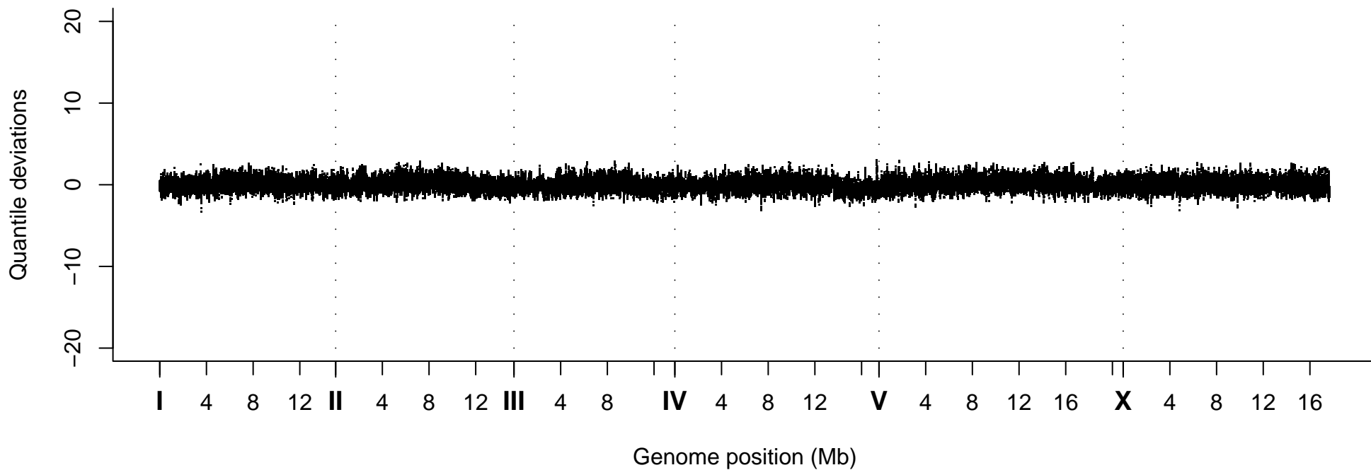
Quantile Deviations, Strain VC20062
