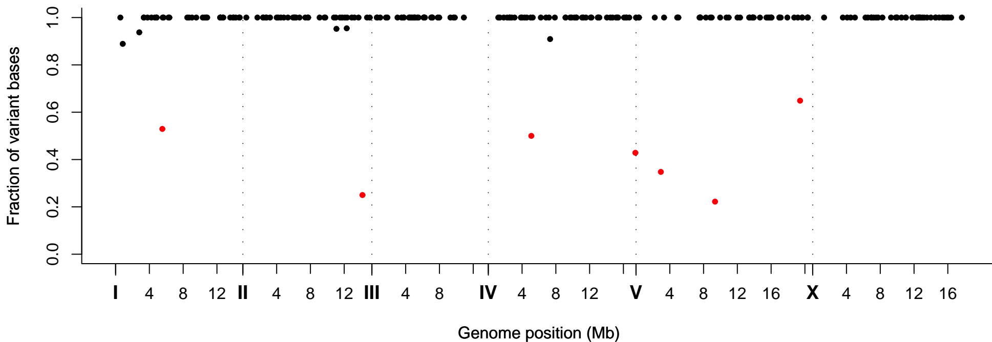
Fraction of Variant Bases at Position, Strain VC20064
