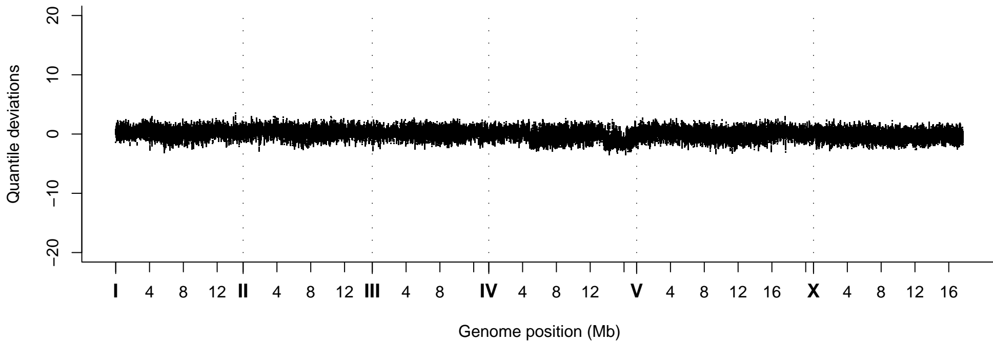
Quantile Deviations, Strain VC20064
