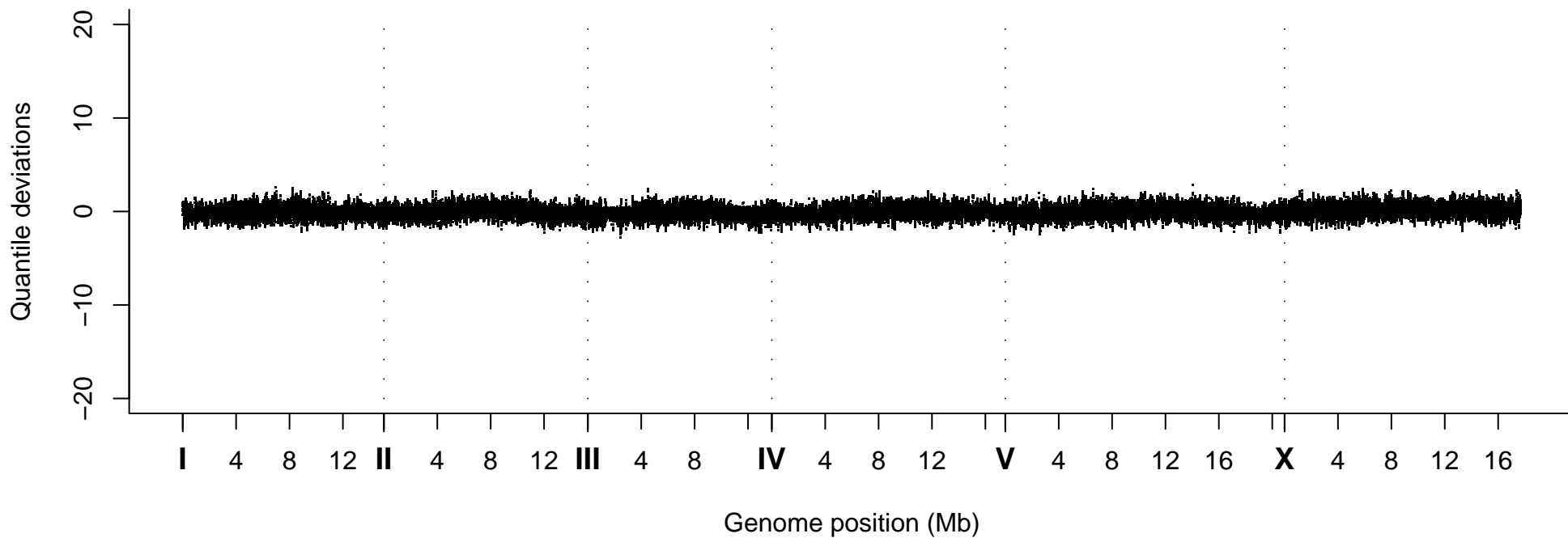
Quantile Deviations, Strain VC20070
