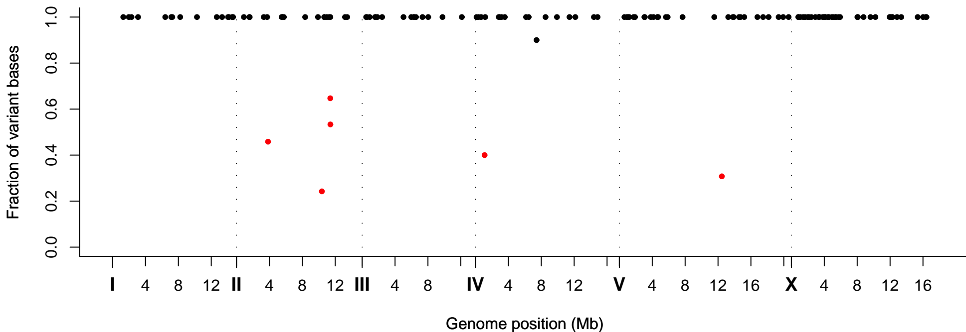
Fraction of Variant Bases at Position, Strain VC20070
