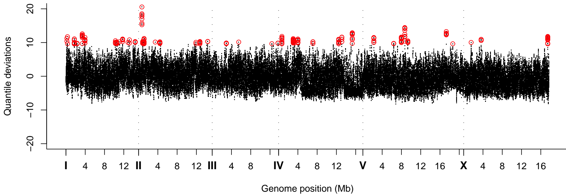
Quantile Deviations, Strain VC20073
