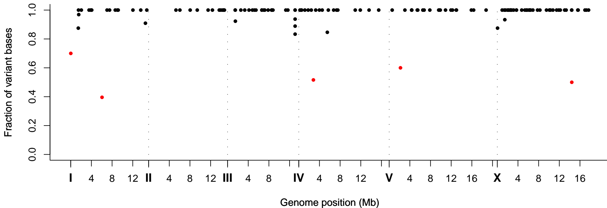
Fraction of Variant Bases at Position, Strain VC20073
