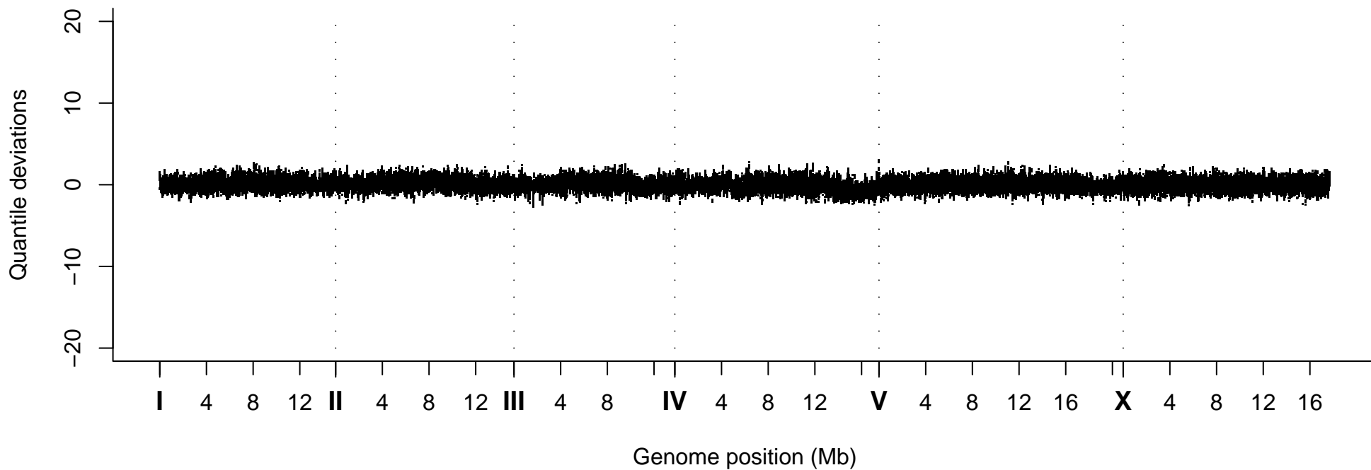
Quantile Deviations, Strain VC20075
