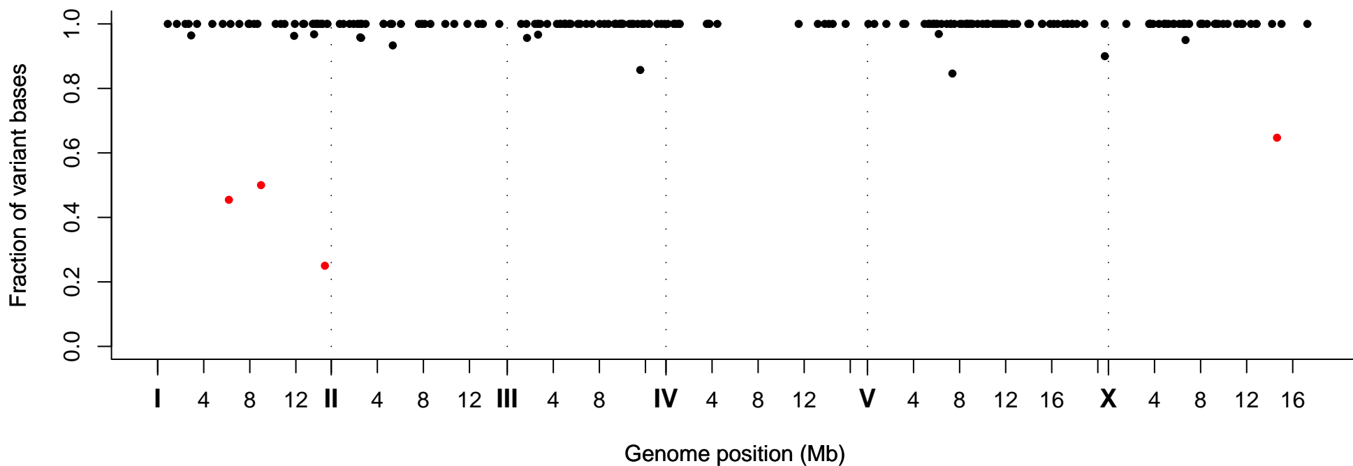
Fraction of Variant Bases at Position, Strain VC20076
