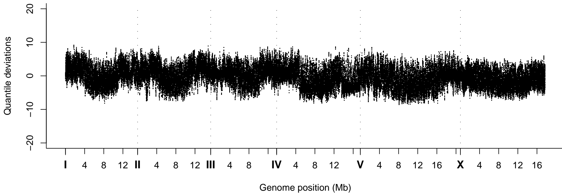
Quantile Deviations, Strain VC20076
