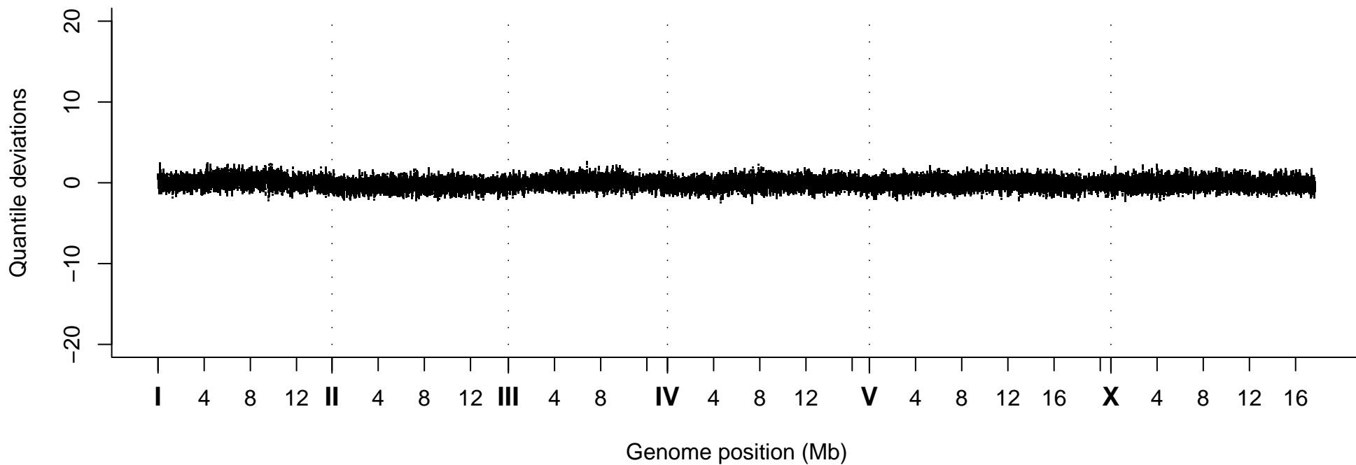
Quantile Deviations, Strain VC20079
