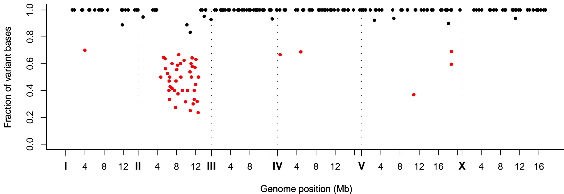
Fraction of Variant Bases at Position, Strain VC20079
