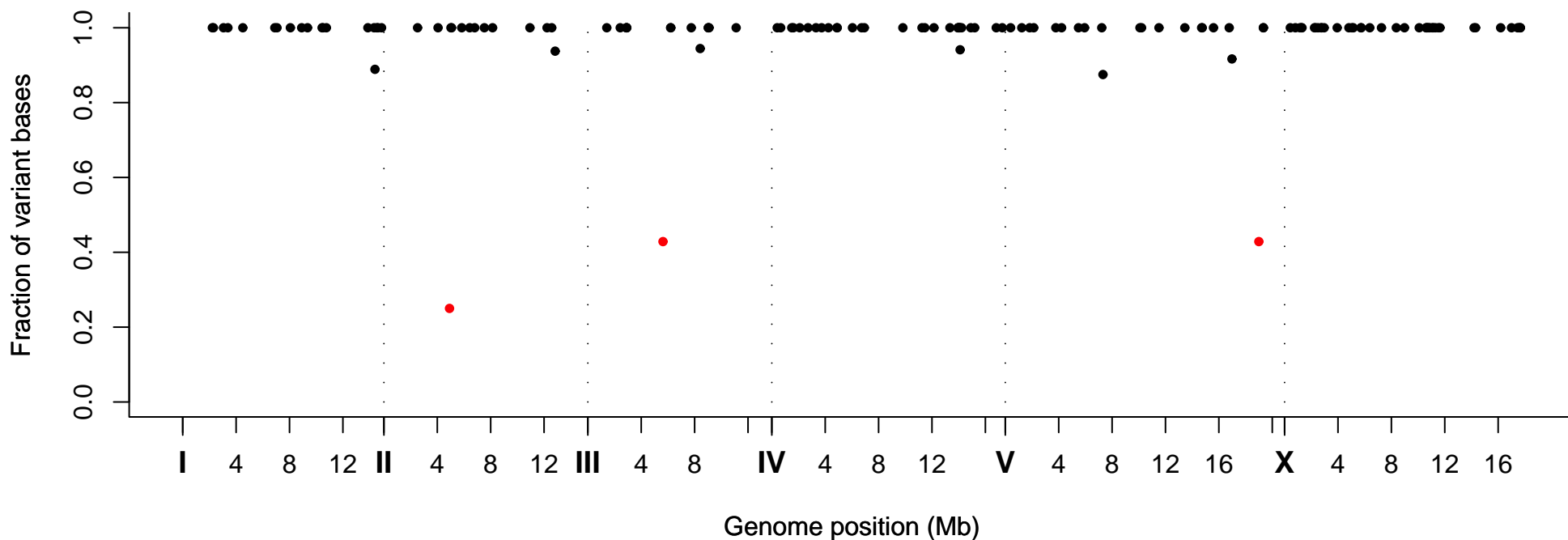
Fraction of Variant Bases at Position, Strain VC20081
