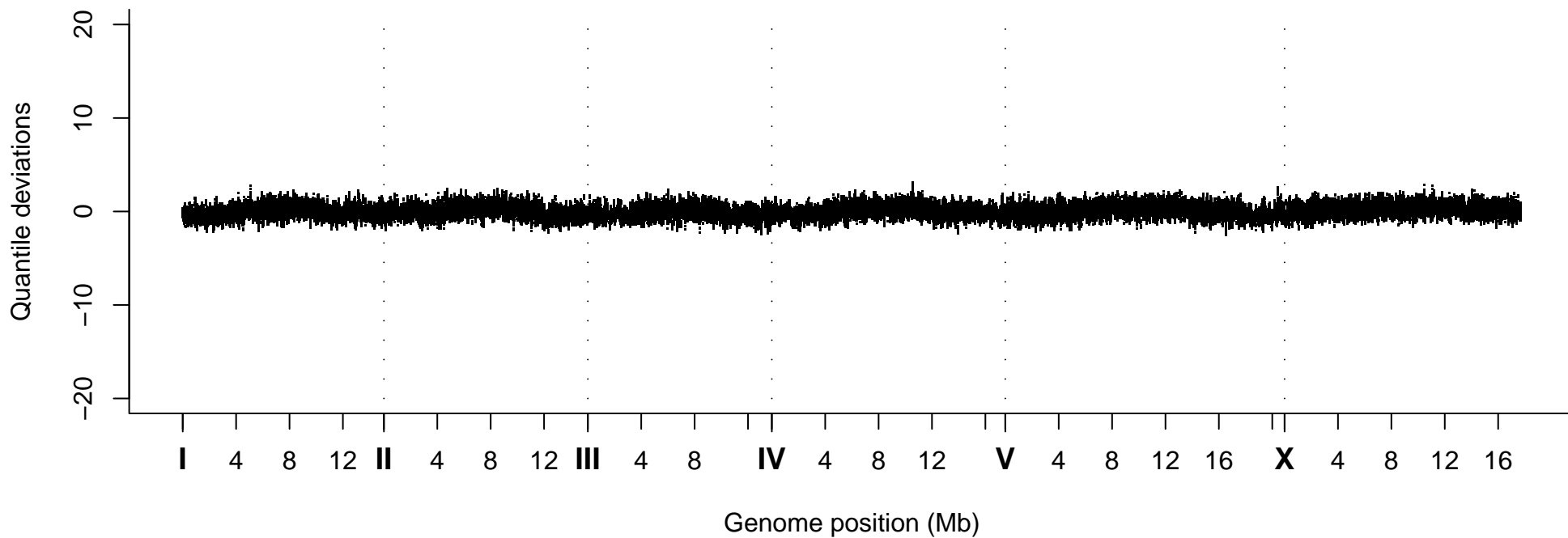
Quantile Deviations, Strain VC20081
