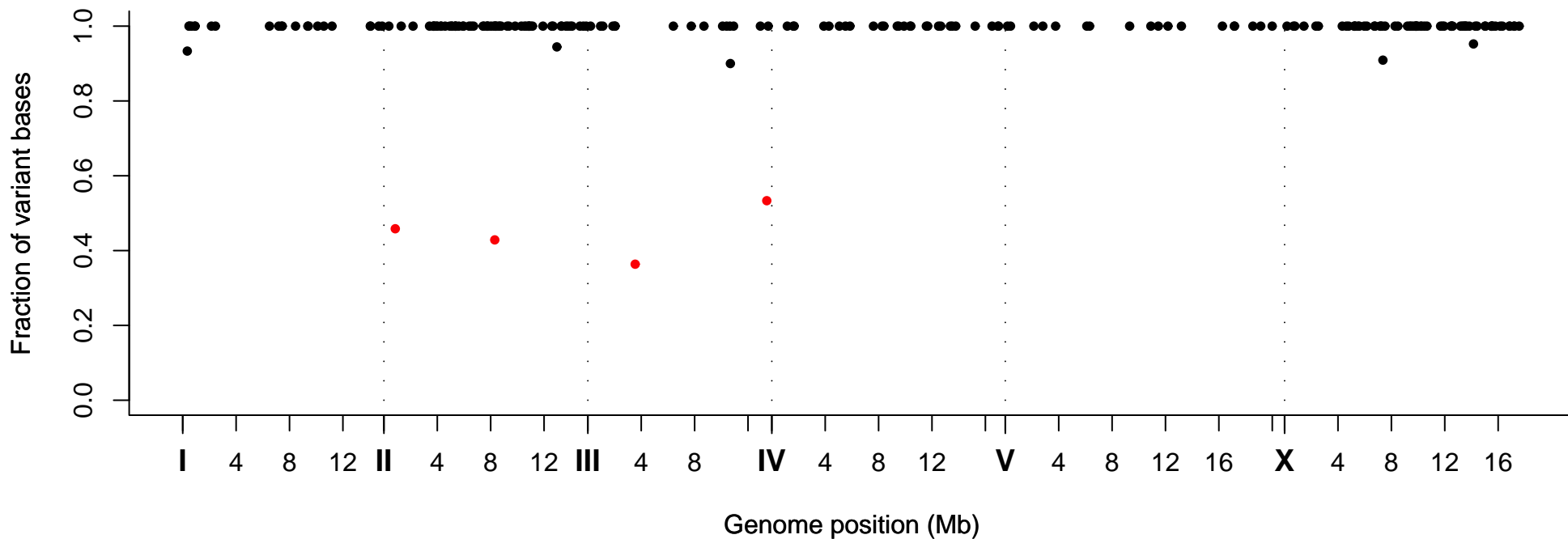
Fraction of Variant Bases at Position, Strain VC20090
