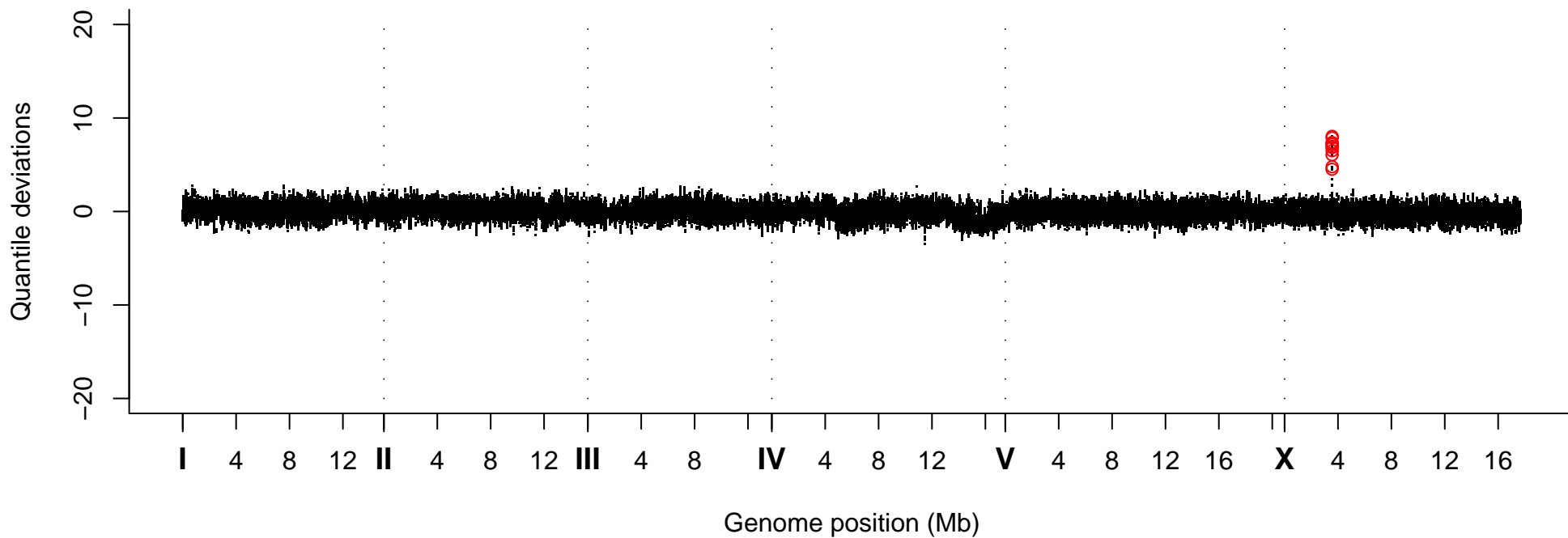
Quantile Deviations, Strain VC20090
