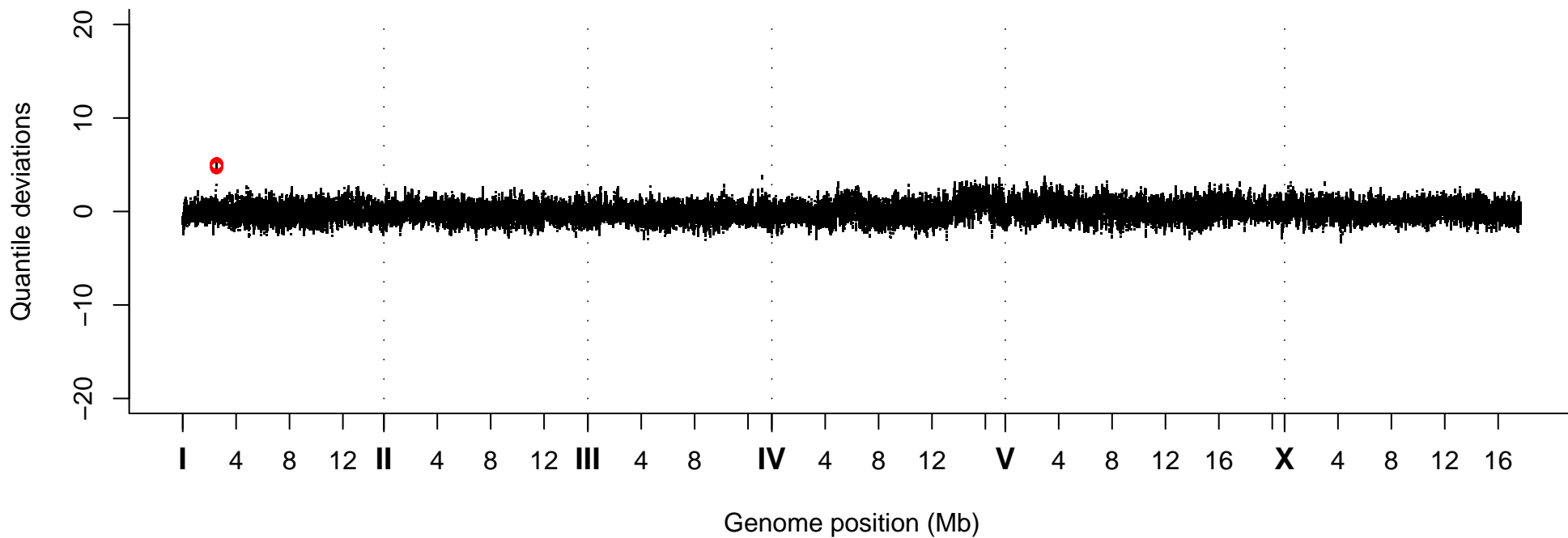
Quantile Deviations, Strain VC20103
