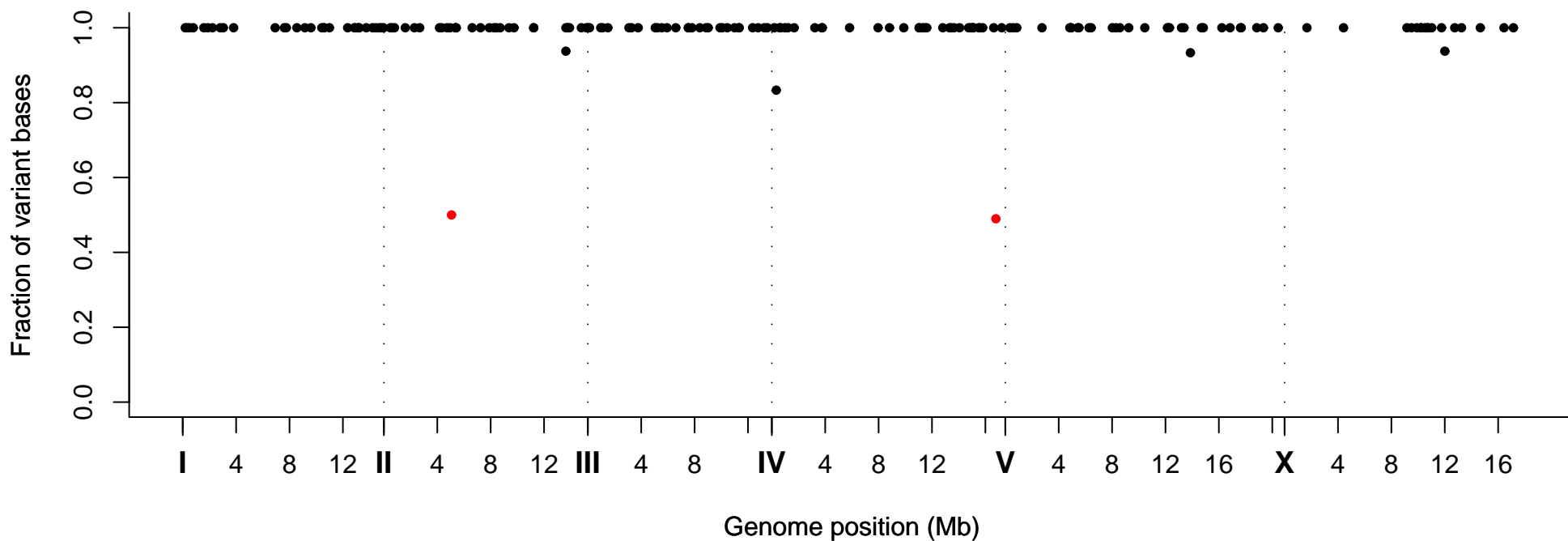
Fraction of Variant Bases at Position, Strain VC20103
