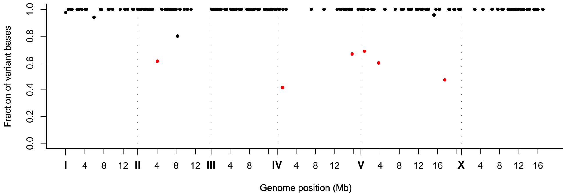
Fraction of Variant Bases at Position, Strain VC20110
