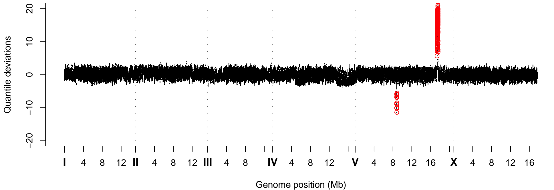
Quantile Deviations, Strain VC20110
