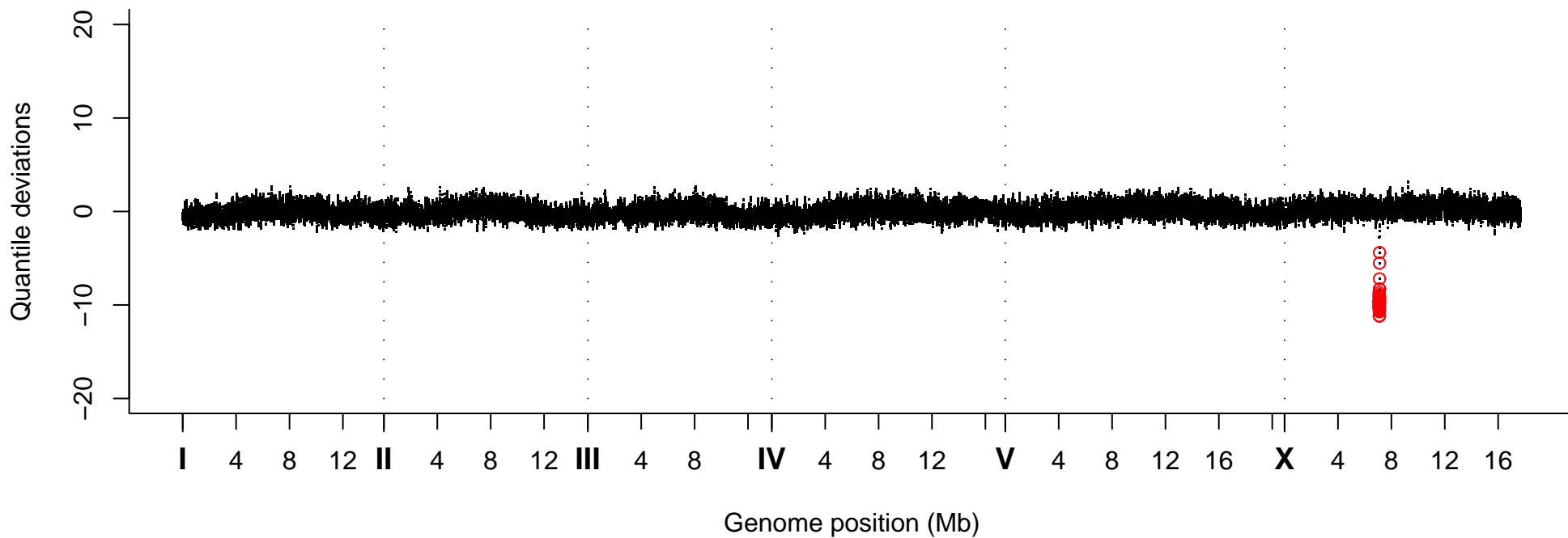
Quantile Deviations, Strain VC20131
