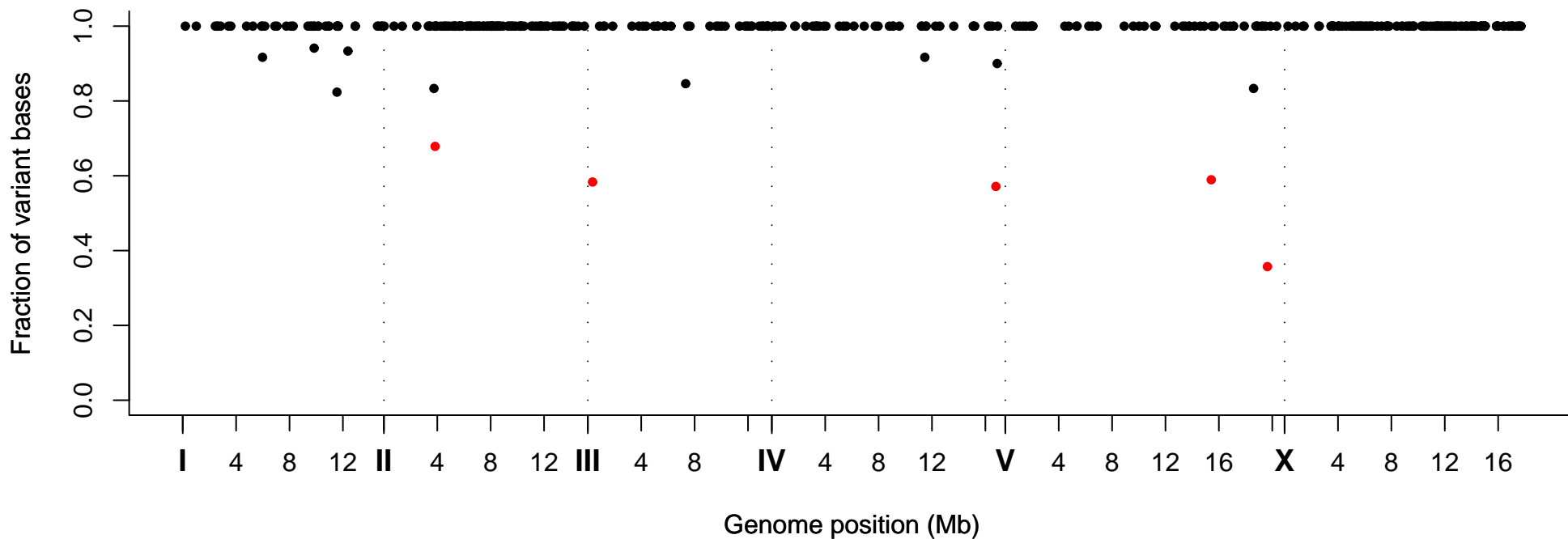
Fraction of Variant Bases at Position, Strain VC20131
