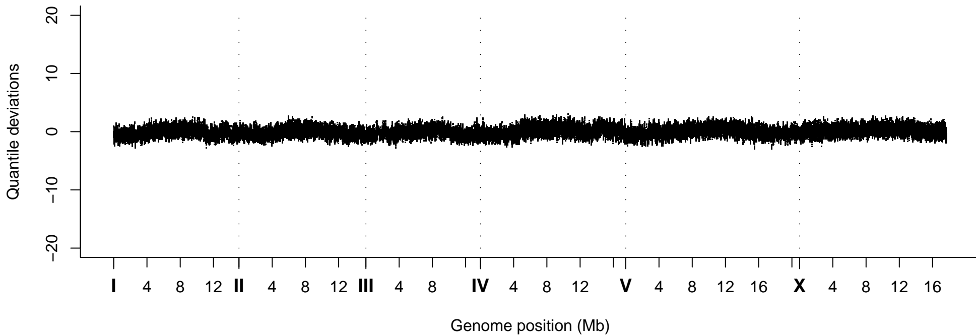
Quantile Deviations, Strain VC20132
