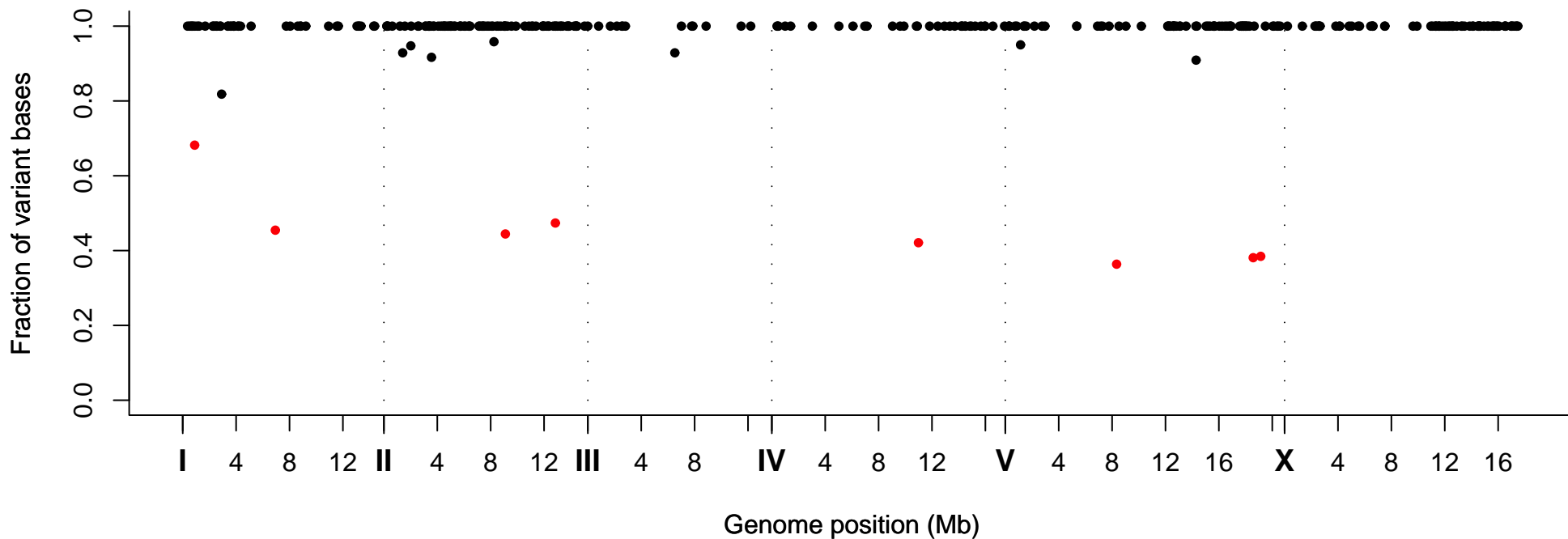
Fraction of Variant Bases at Position, Strain VC20132
