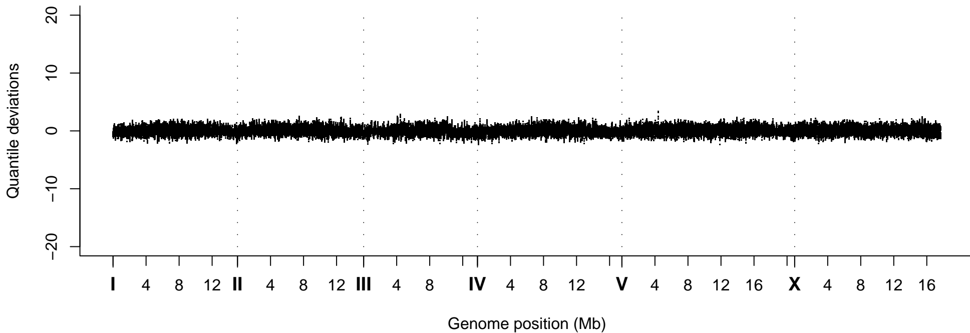
Quantile Deviations, Strain VC20134
