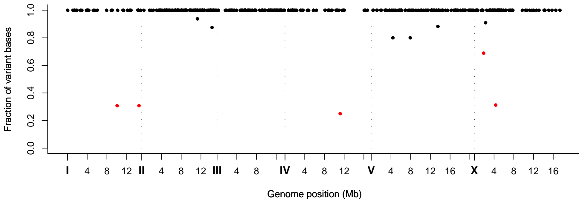
Fraction of Variant Bases at Position, Strain VC20134
