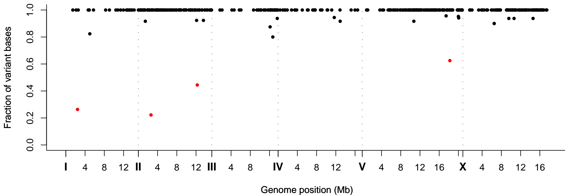
Fraction of Variant Bases at Position, Strain VC20138
