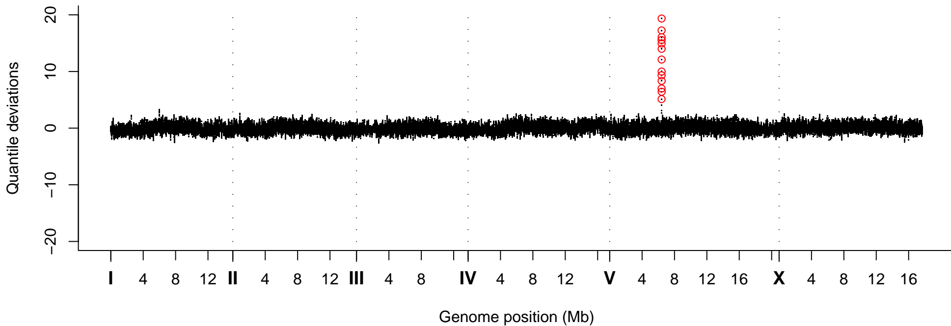
Quantile Deviations, Strain VC20138
