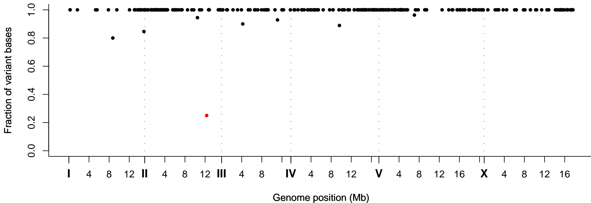
Fraction of Variant Bases at Position, Strain VC20140
