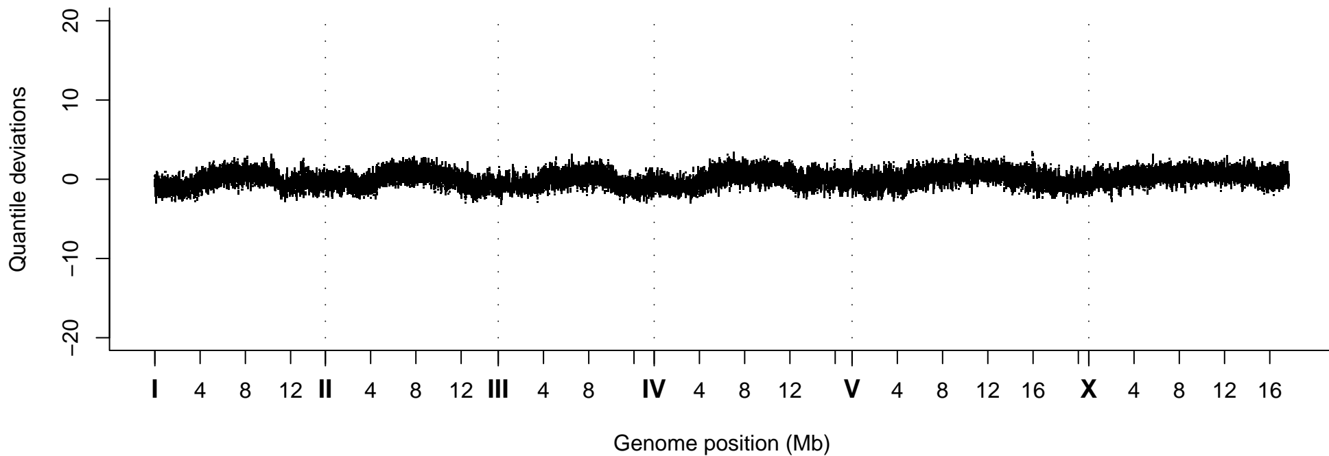
Quantile Deviations, Strain VC20140
