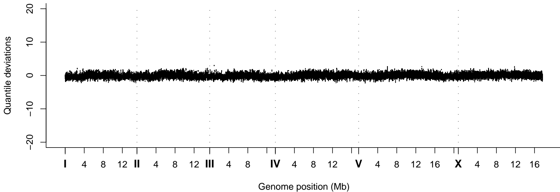
Quantile Deviations, Strain VC20144
