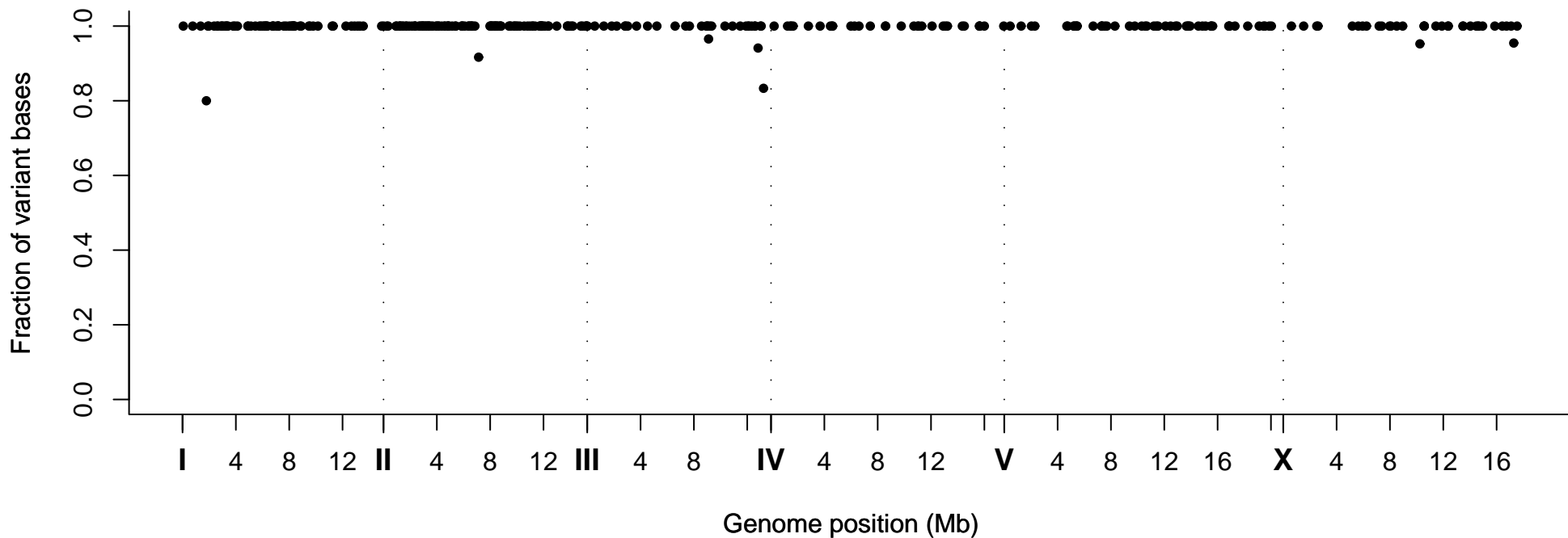
Fraction of Variant Bases at Position, Strain VC20144
