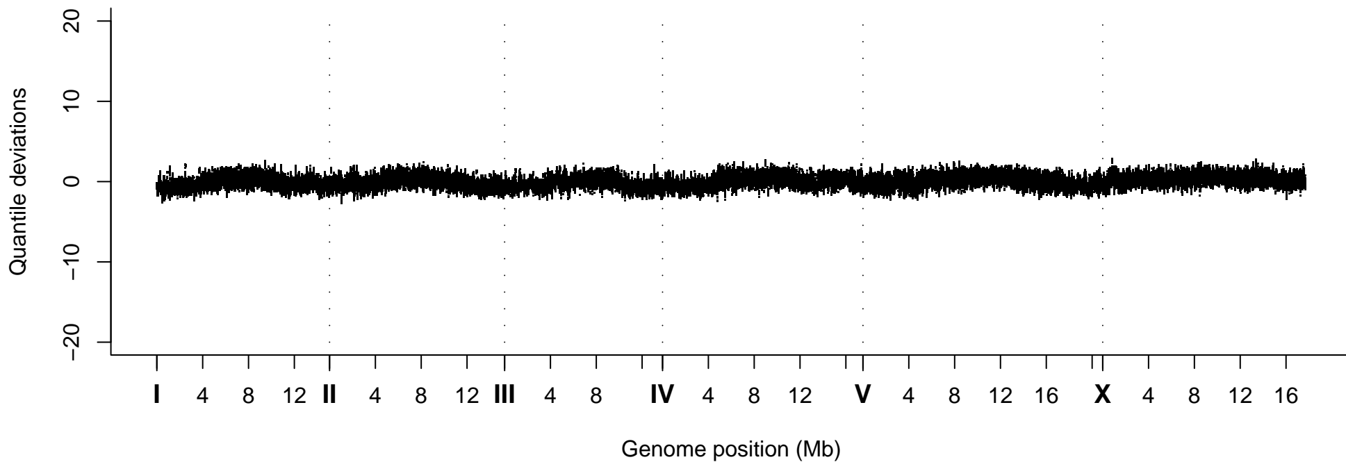
Quantile Deviations, Strain VC20148
