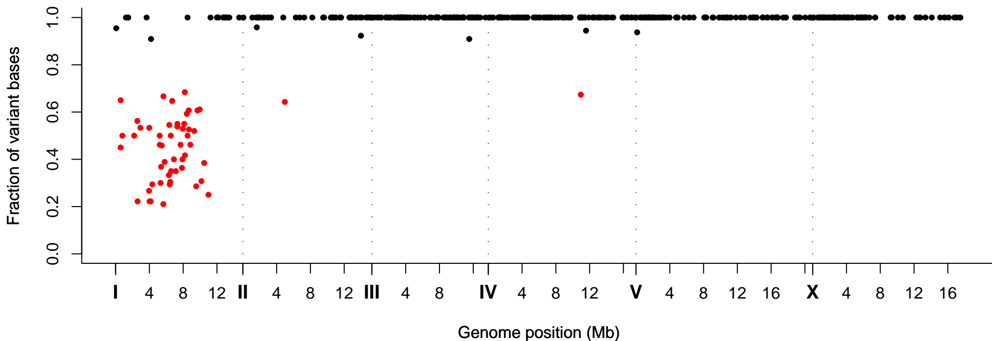
Fraction of Variant Bases at Position, Strain VC20148
