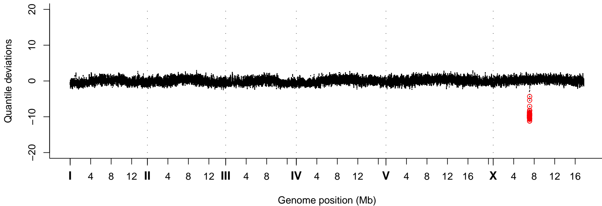
Quantile Deviations, Strain VC20152
