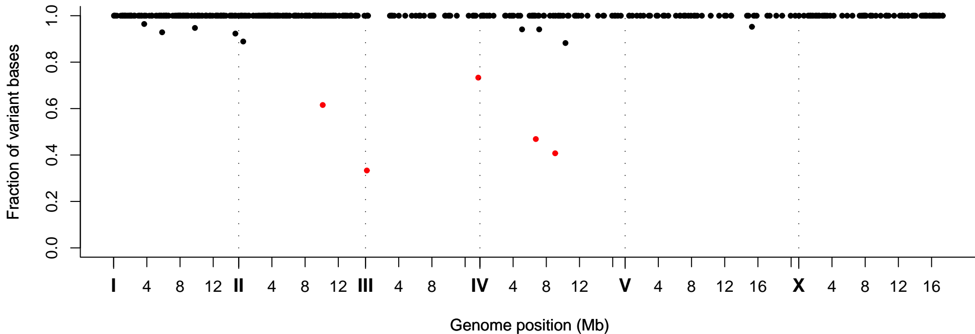
Fraction of Variant Bases at Position, Strain VC20152
