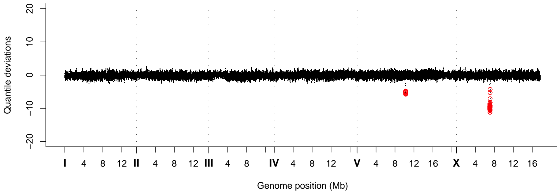
Quantile Deviations, Strain VC20156
