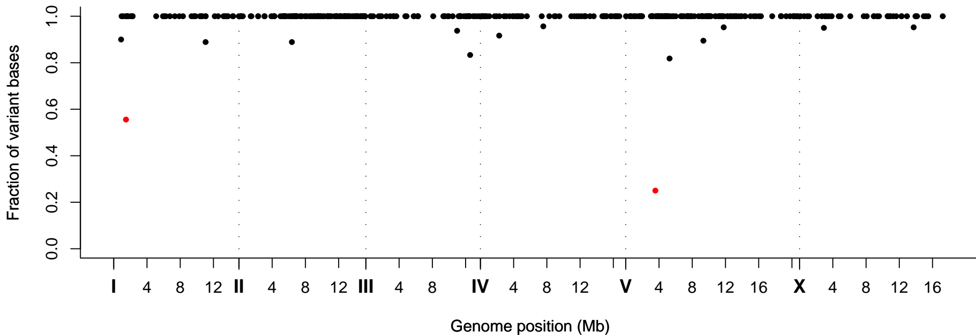
Fraction of Variant Bases at Position, Strain VC20156
