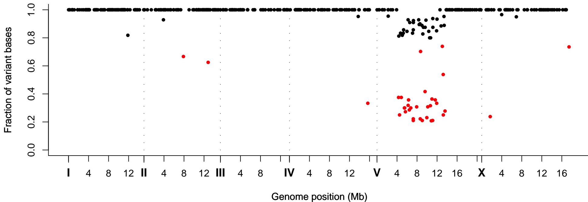
Fraction of Variant Bases at Position, Strain VC20161
