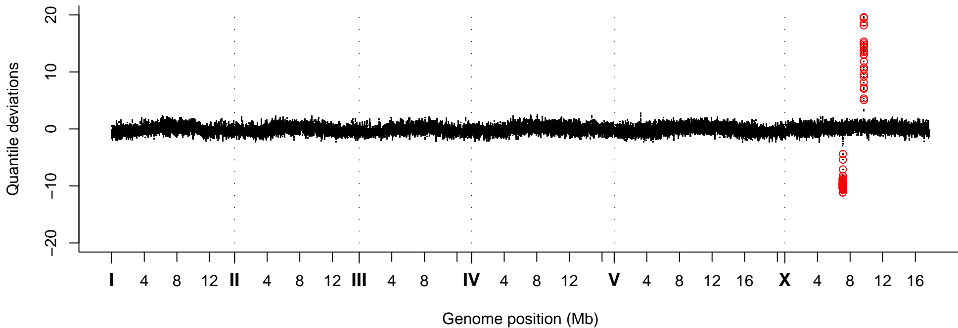
Quantile Deviations, Strain VC20161
