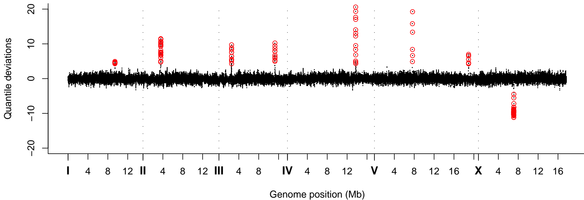
Quantile Deviations, Strain VC20168
