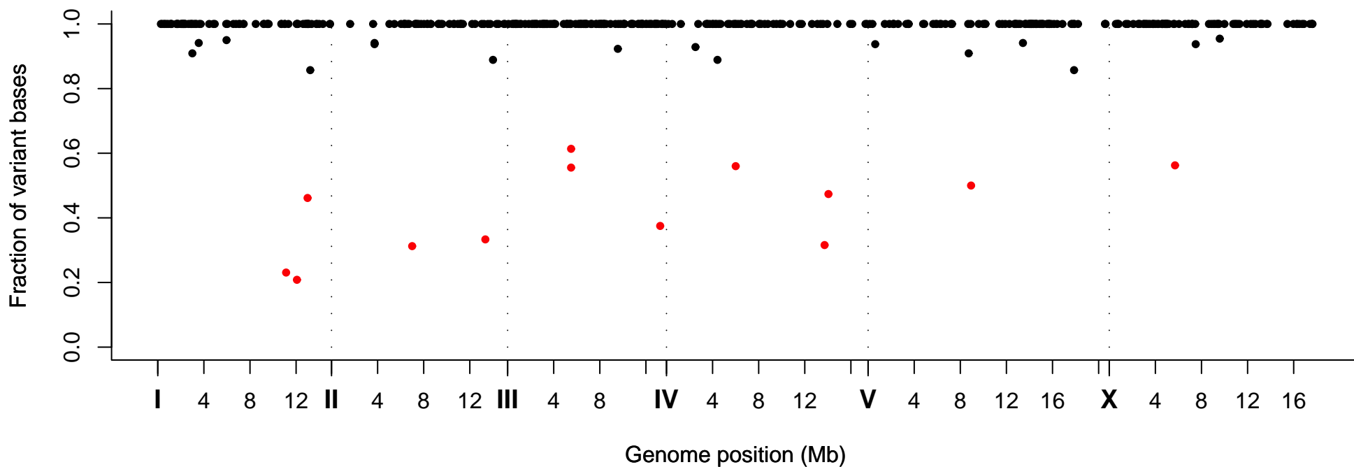
Fraction of Variant Bases at Position, Strain VC20168
