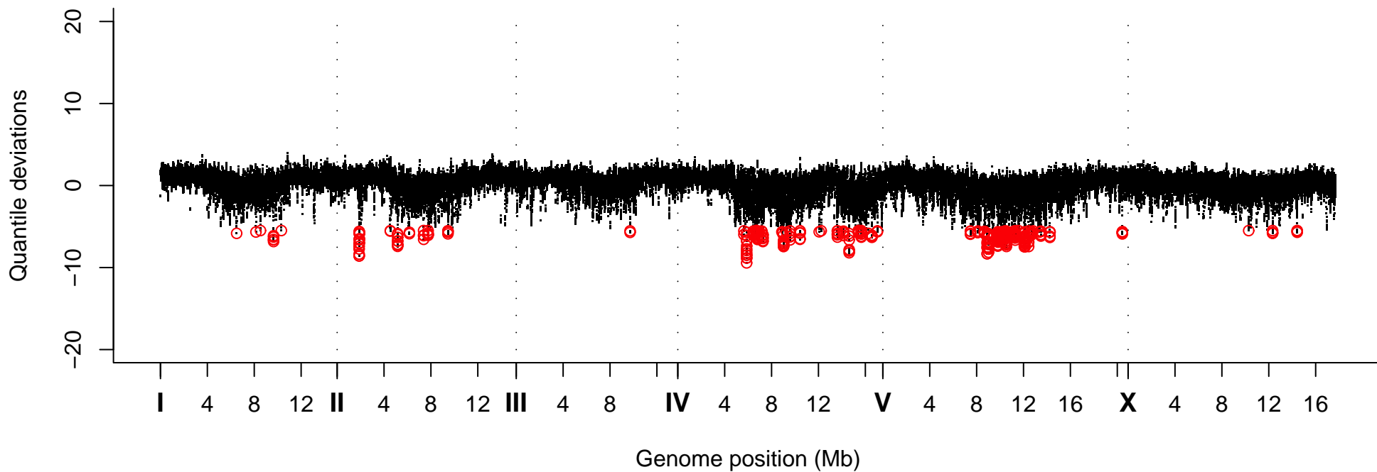
Quantile Deviations, Strain VC20172
