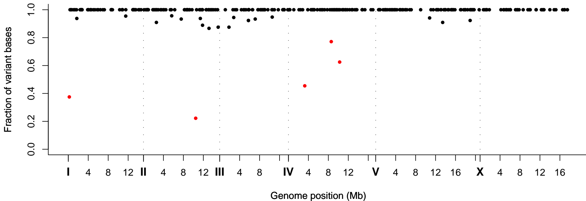
Fraction of Variant Bases at Position, Strain VC20172
