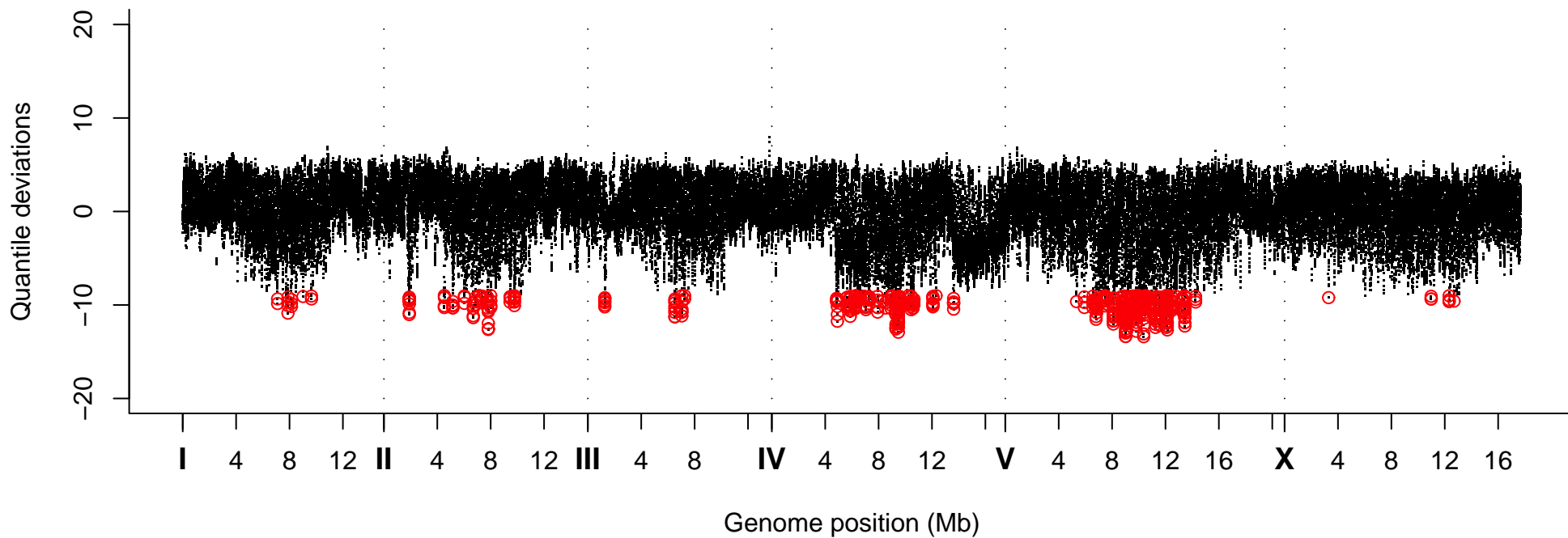
Quantile Deviations, Strain VC20173
