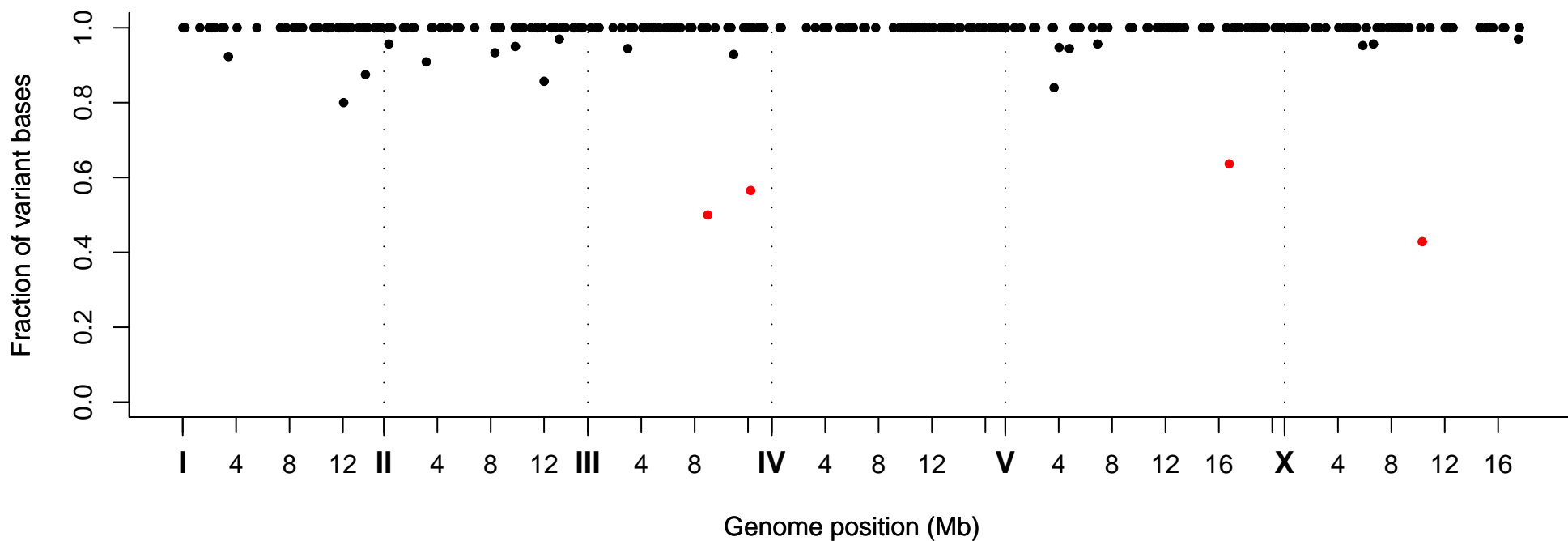
Fraction of Variant Bases at Position, Strain VC20173
