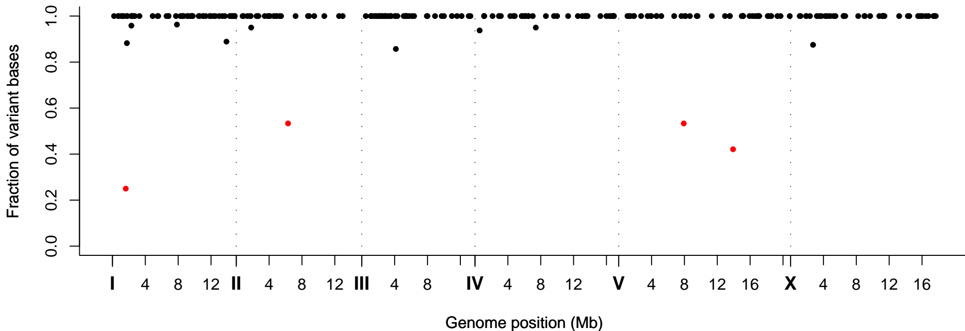
Fraction of Variant Bases at Position, Strain VC20174
