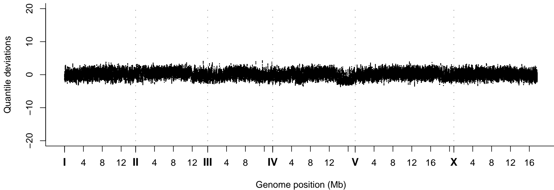
Quantile Deviations, Strain VC20174
