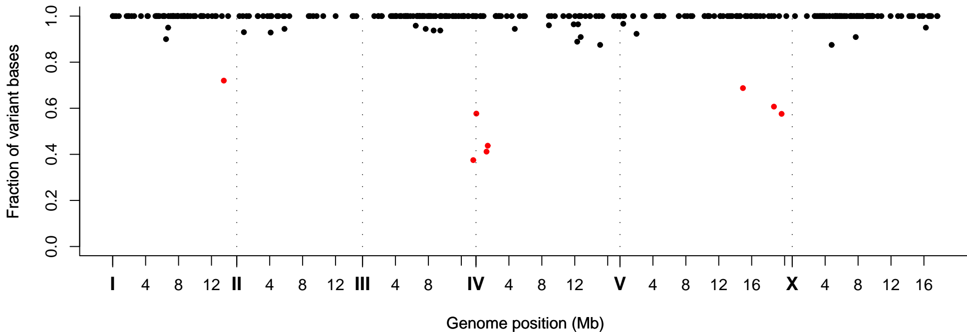
Fraction of Variant Bases at Position, Strain VC20181
