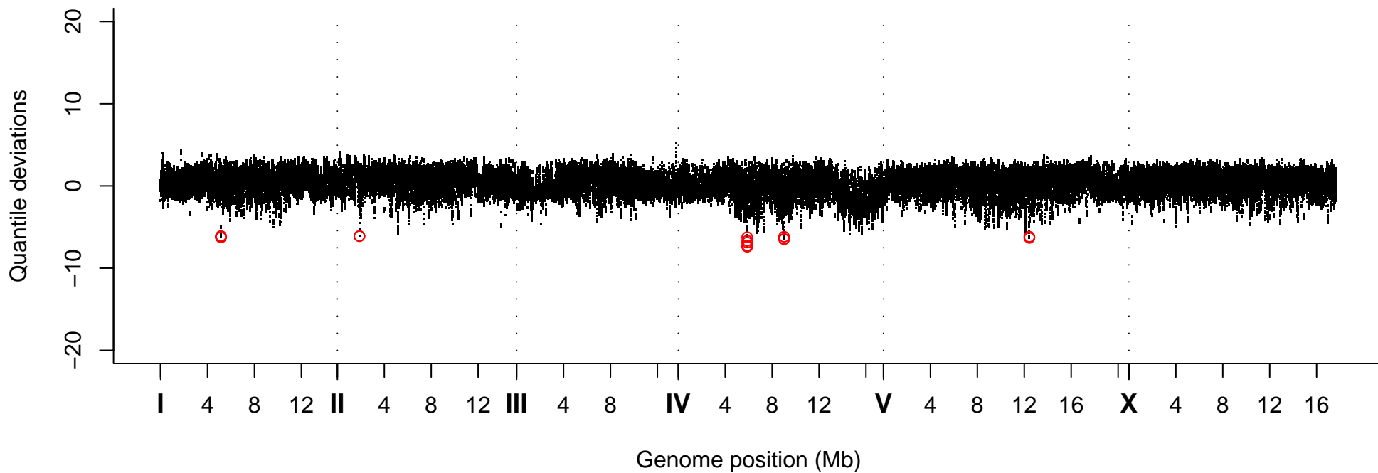
Quantile Deviations, Strain VC20181
