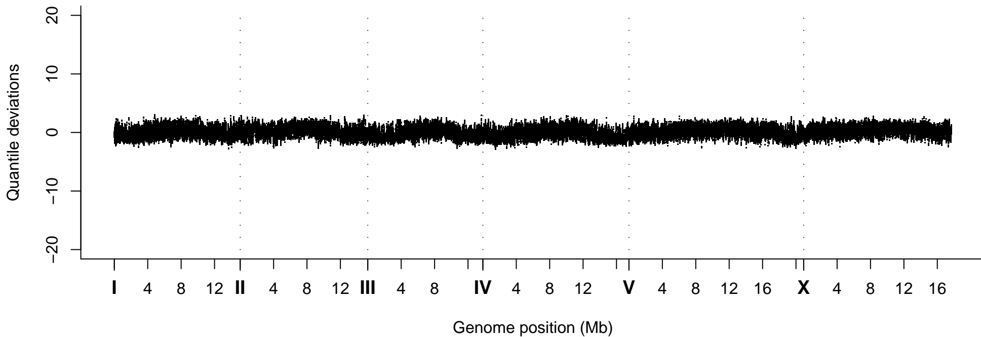
Quantile Deviations, Strain VC20187
