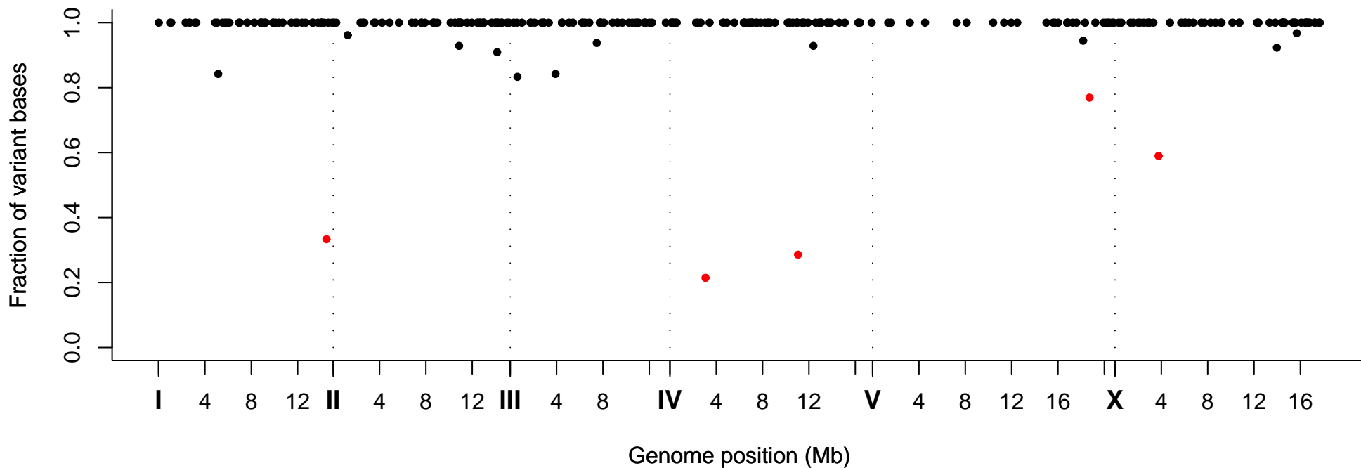
Fraction of Variant Bases at Position, Strain VC20187
