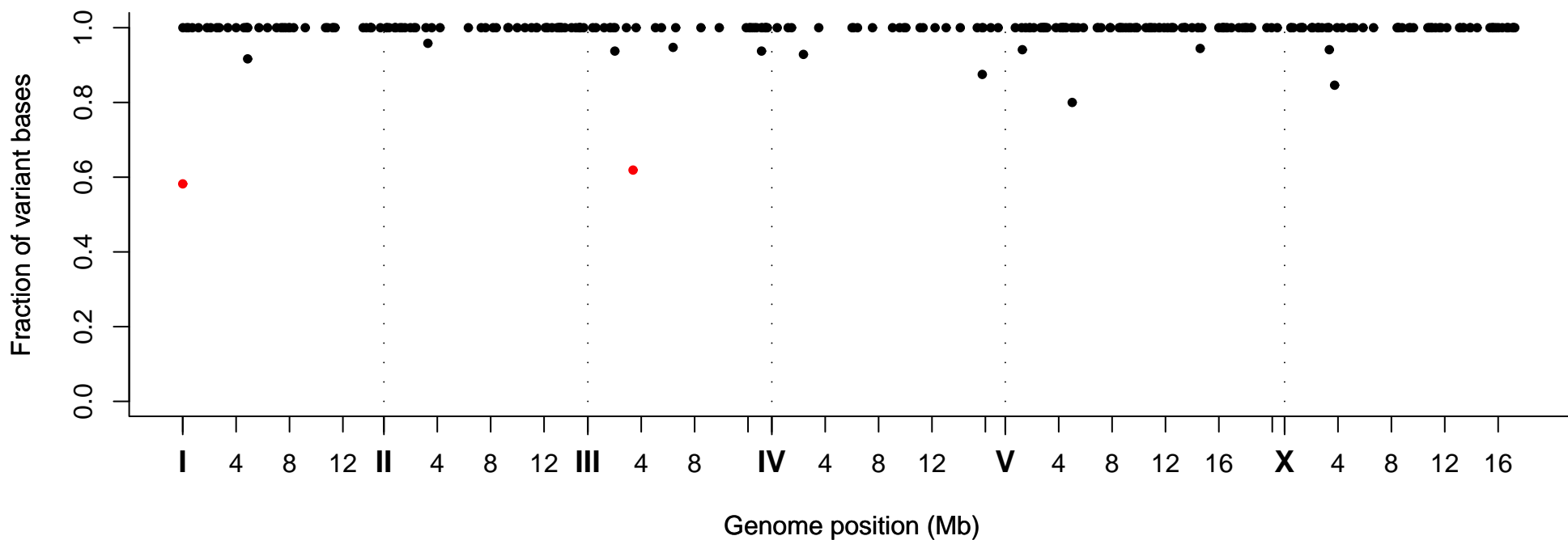
Fraction of Variant Bases at Position, Strain VC20188
