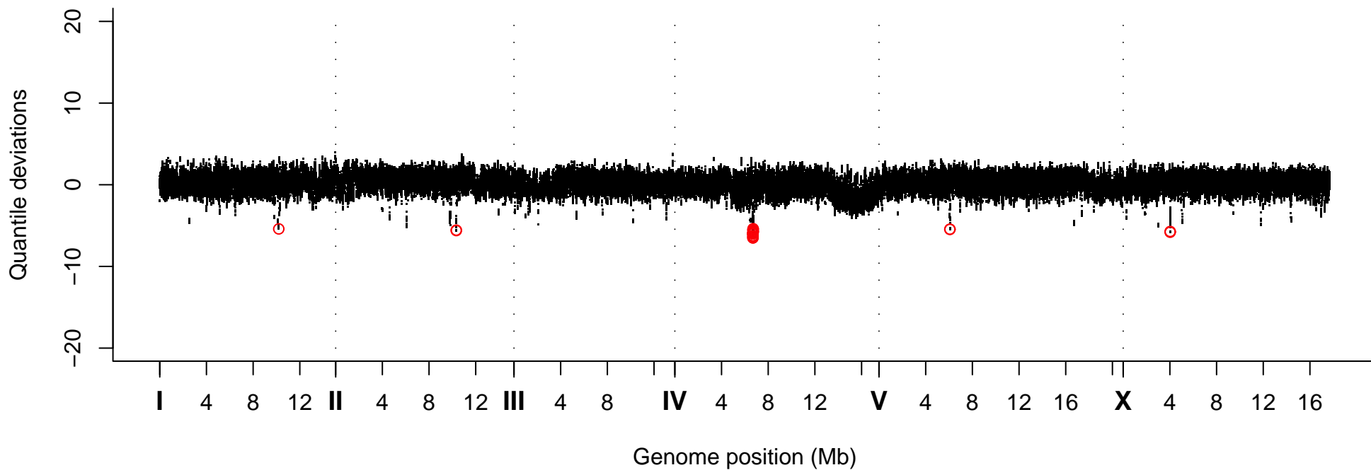
Quantile Deviations, Strain VC20188
