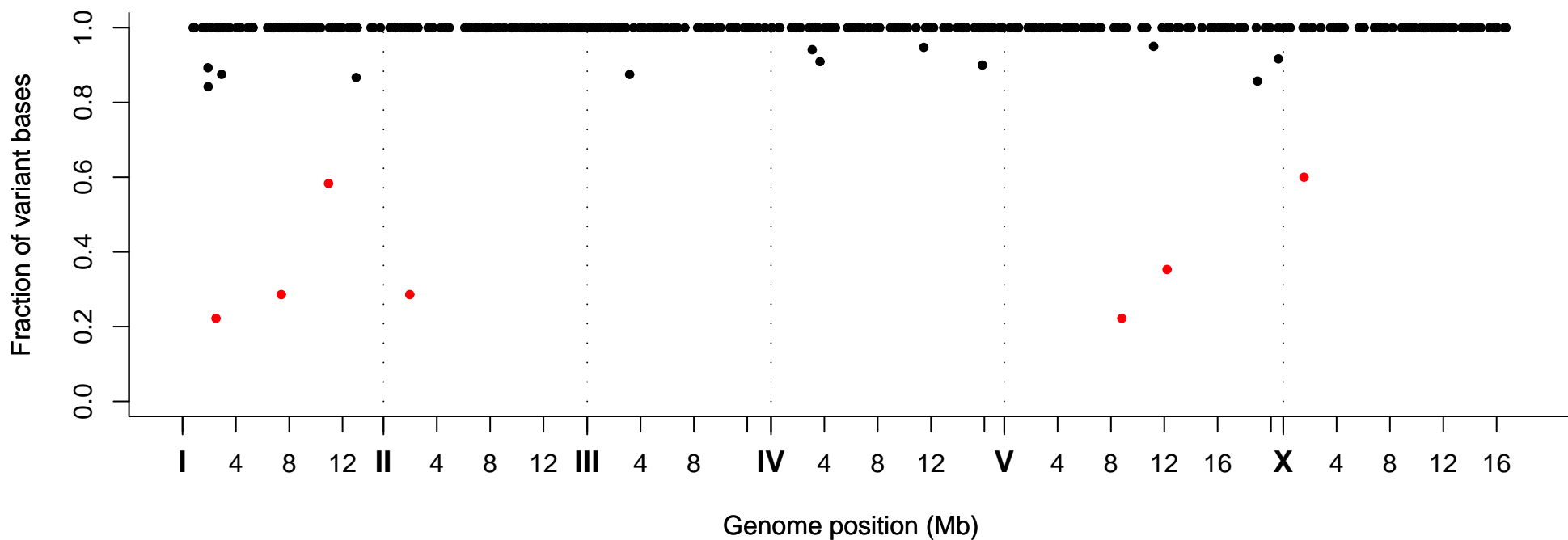
Fraction of Variant Bases at Position, Strain VC20190
