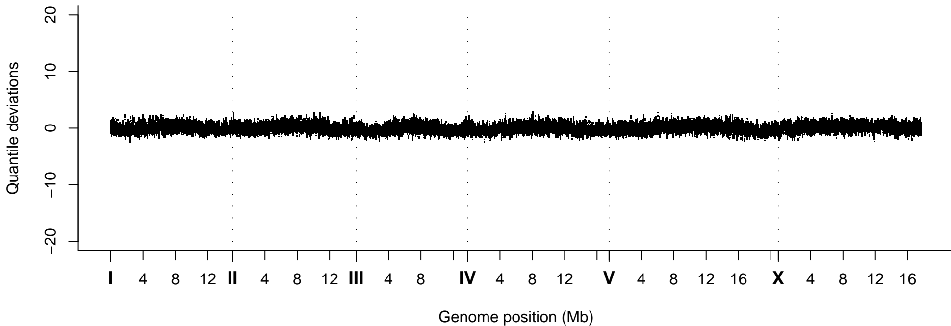
Quantile Deviations, Strain VC20190
