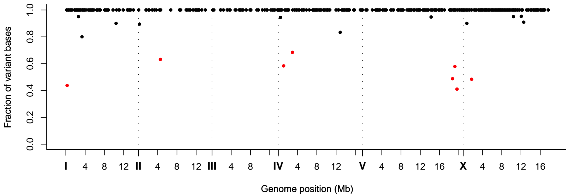
Fraction of Variant Bases at Position, Strain VC20191
