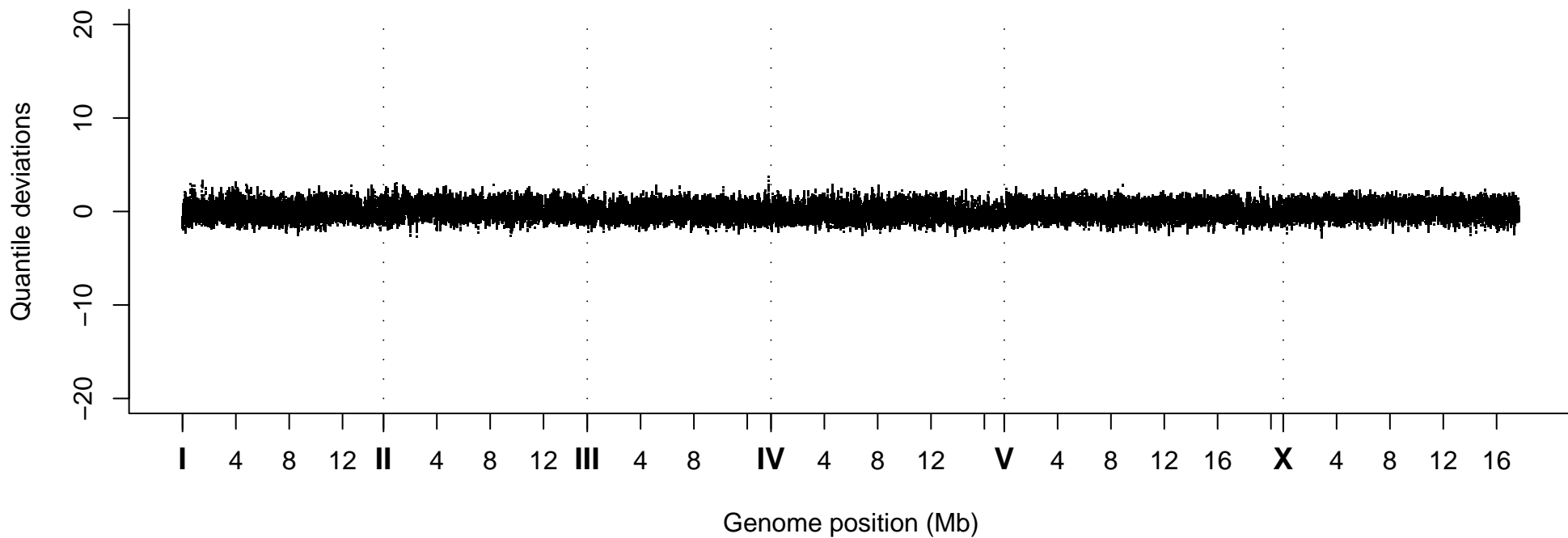
Quantile Deviations, Strain VC20191
