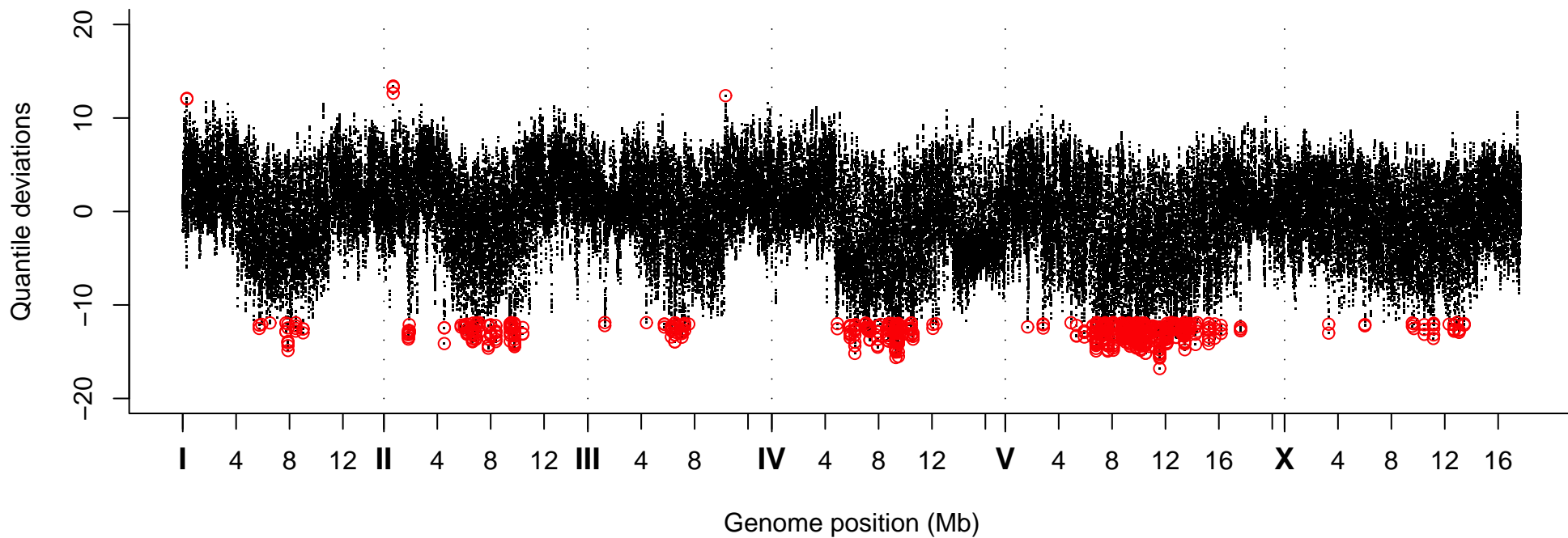
Quantile Deviations, Strain VC20201
