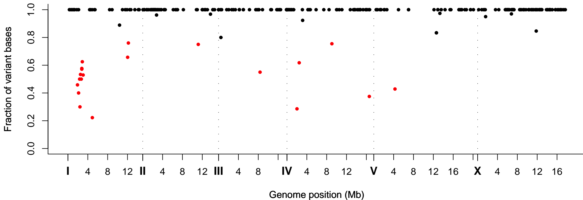
Fraction of Variant Bases at Position, Strain VC20201
